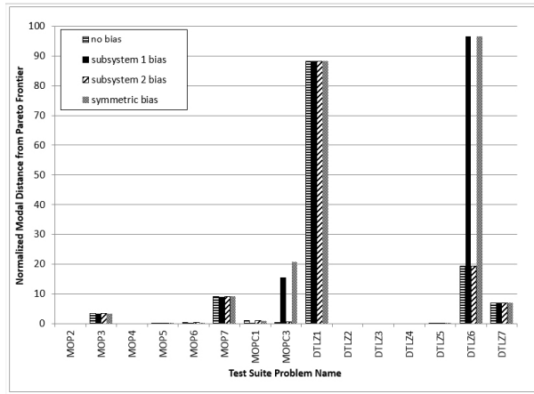
Fig. 8. Normalized Distance to Pareto Frontier for Asymmetric Decreasing Bias Conditions
