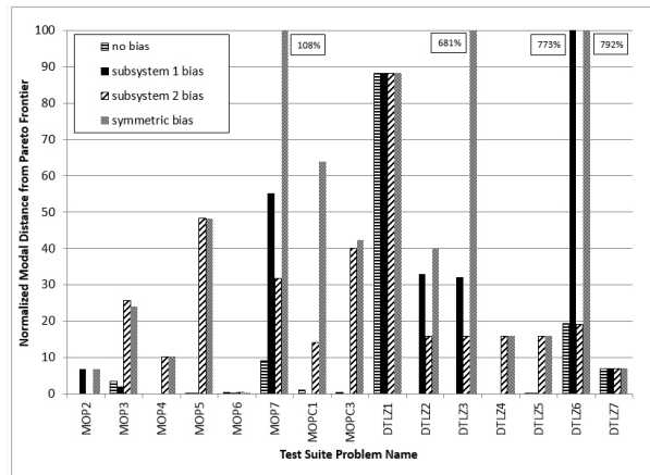
Fig. 7. Normalized Distance to Pareto Frontier for Asymmetric Constant Bias Conditions
