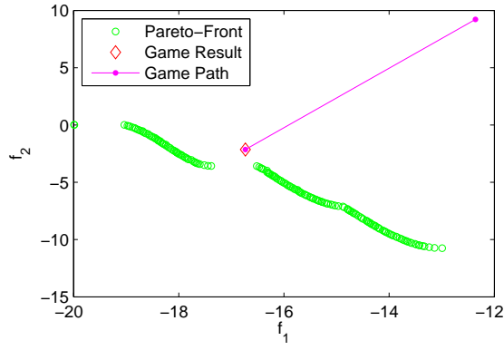
Fig. 5. Solution path in the static bias condition. b = 1.3
