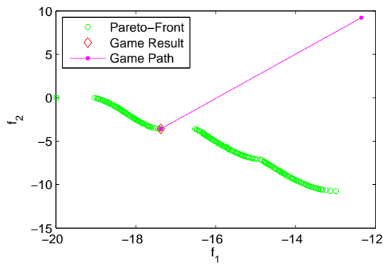
Fig. 4. Solution path in the no bias condition. b = 0
