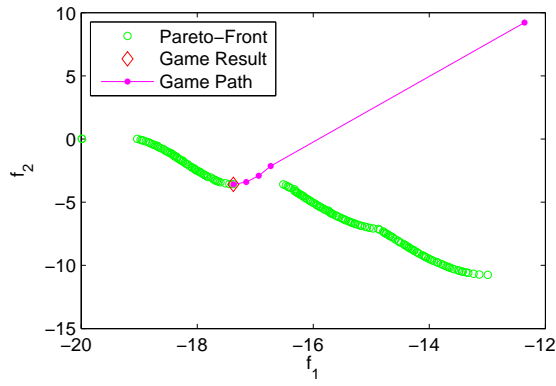
Fig. 6. Solution path in the decreasing bias condition. b = 1.3 - .1 * i
