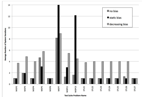
Fig. 3. Average number of system iterations for all three test conditions
