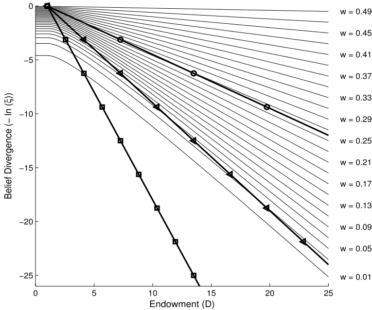
Fig. 1. Survival. This figure illustrates survival results in Examples 3.1 and 3.2. We set \lambda = 1 . We plot the aggregate endowment D on the horizontal axis, and the negative of the log of relative belief density, -\ln(\xi) , on the vertical axis. Solid lines are the level curves for the consumption share of agent \mathbb{B} , so that each solid line plots pairs (D, \ln(\xi)) that give rise to a given consumption share w . These pairs can be found by fixing w and plotting the value of \ln(\xi) as a function of D , with the function given by the Pareto optimality condition (8). Labels for agent \mathbb{B} 's consumption share are shown along the right margin. The marked lines show the median path ( Z_t = 0 ) of (D_t, \ln(\xi_t)) for each case in Example 3.1. We choose \delta = 0.5 and set \mu in cases (i), (ii), and (iii) to \delta^2 , \delta^2/4 , and \delta^2/2 respectively. We mark the corresponding median paths with circles, squares, and triangles.
