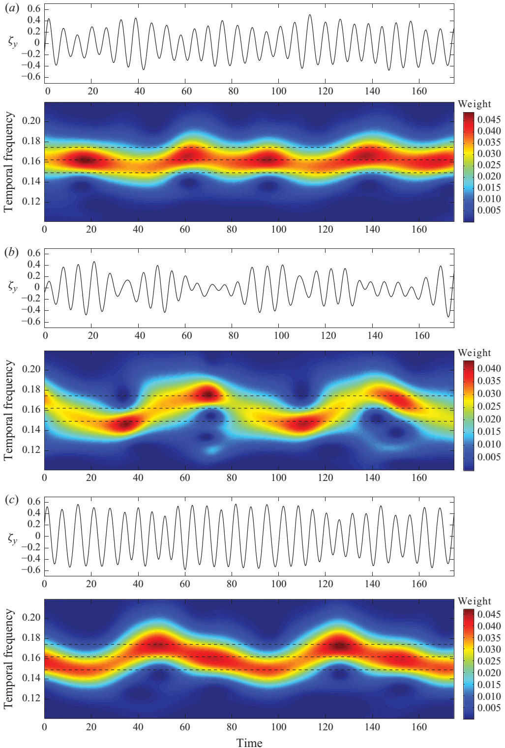
FIGURE 8. Selected cross-flow displacement time series (upper part) and corresponding frequency content as a function of time (scalogram, lower part) in the case Re_m = 330 at (a) z=94 , (b) z=44 and (c) z=7.5 . The dashed lines denote the predominant frequencies identified in figure 6(c).
