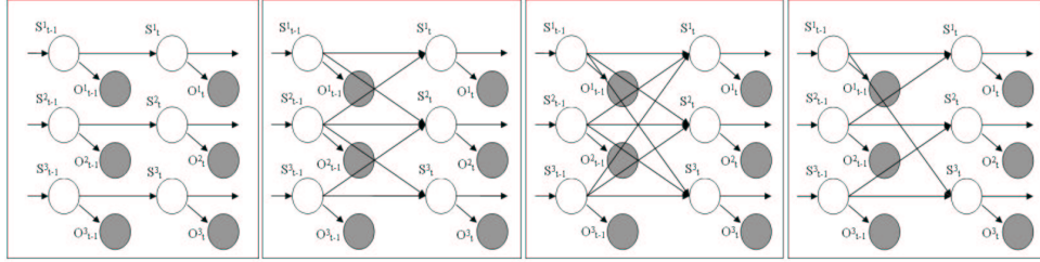
Figure 1: Four types of Dynamic Bayesian Networks: PaHMM, CHMM, FHMM and DML-HMM.
