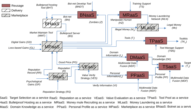
Fig. 5. Marketplace and Gain Reuse. “Marketplace” refers to the services to enable the trade for benefit realization while “Reusage” refers to the services that reuse the digital gains from previous successful cyber attacks to facilitate further attacks.
