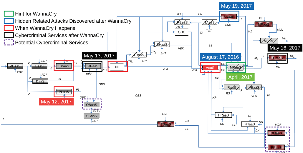
Fig. 4. Understand WannaCry cyber attack evolution using the cybercriminal service ecosystem framework.
