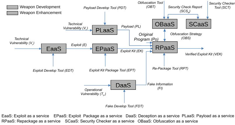
Fig. 3. Exploitation Development Service (EKaaS). “Weapon development” means the service is related to transfer the vulnerability into the weapon that can be used for attack. “Weapon enhancement” means the service is used to improve the effectiveness of the weapons.
