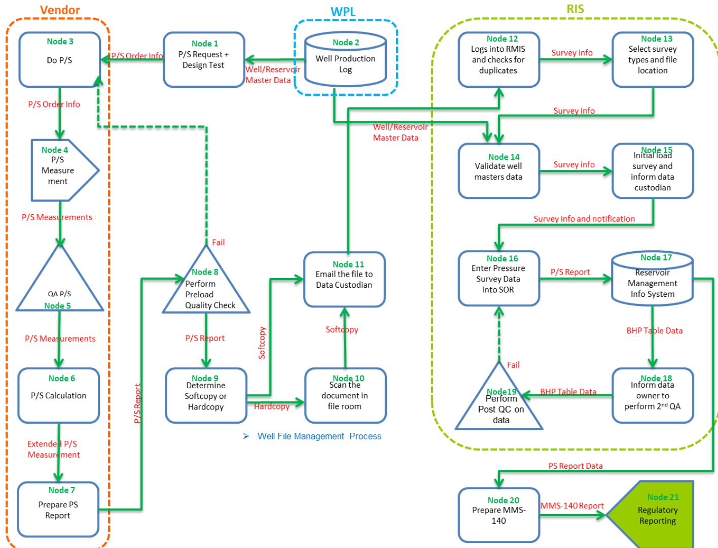
Figure 13: IPMAP of RIS
