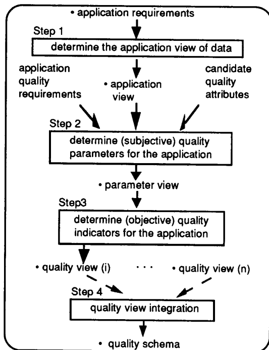
Figure 2: The process of data quality modeling
