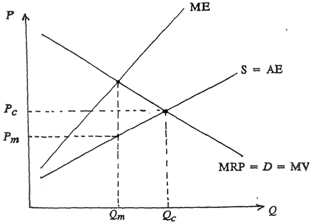
Figure 4: Monopsony Power
