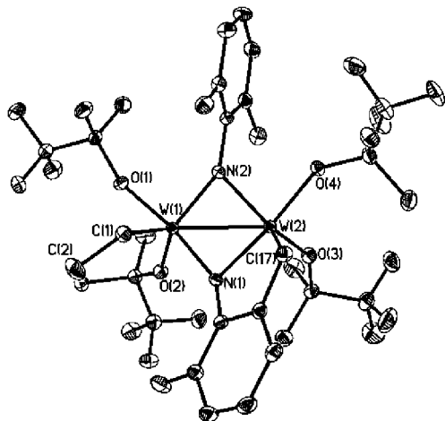
Figure 3. Thermal ellipsoid plot of (\text{OCMe}_2\text{CF}_3)_2(\text{Et})\text{W}(\mu\text{-NAr}')(\mu\text{-N-2-CH}_2\text{-6-MeC}_6\text{H}_3)\text{W}(\text{OCMe}_2\text{CF}_3)_2 .
