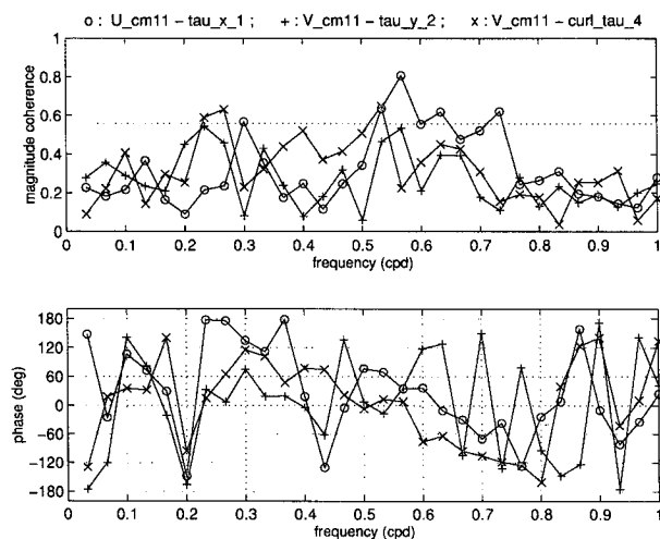
FIG. 9. Coherence spectra of 80-m currents at mooring 1 ( 63.25^\circ\text{N} , 12^\circ\text{W} ) and atmospheric variables; (top) coherence magnitude, (bottom) coherence phase. Circles correspond to zonal current and zonal wind stress averaged over ( 62.8^\circ-63.8^\circ\text{N} , 11.3^\circ-13.1^\circ\text{W} ), + correspond to meridional current and meridional wind stress averaged over ( 61.8^\circ-62.8^\circ\text{N} , 11.3^\circ-13.1^\circ\text{W} ), and \times 's correspond to meridional current and wind stress curl averaged over ( 60.8^\circ-63.8^\circ\text{N} , 10.3^\circ-15.0^\circ\text{W} ). The 95% level of significance for the coherence amplitude is indicated by the dotted line. Positive phase indicates that the first variable leads the second.
