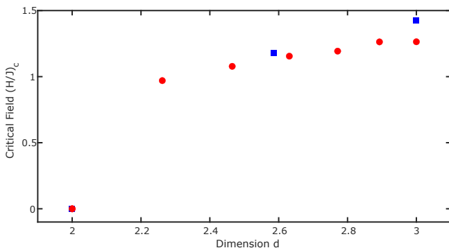
FIG. 6. The calculated zero-temperature critical fields with respect to spatial dimension d , for the b = 2 (squares) and b = 3 (circles) hierarchical models.
