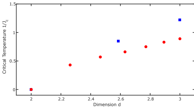
FIG. 5. The calculated zero-field critical temperatures with respect to spatial dimension d , for the b = 2 (squares) and b = 3 (circles) hierarchical models.
