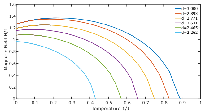
FIG. 3. Six calculated phase diagrams of the random-field Heisenberg model, for d = 2.26, 2.46, 2.63, 2.77, 2.89, 3 (inside to outer curves). The exact solutions of a b = 3 hierarchical lattice yield these results. The calculation shows that no ordering occurs in d = 2 . Starting at d = 2.46 , temperature reentrance occurs and is magnified as d = 3 is approached.
