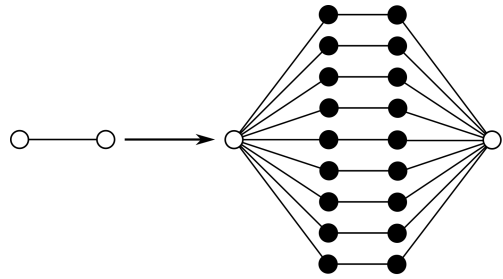
FIG. 1. From Ref.[24]: Construction of a d = 3 hierarchical model used in this study. A hierarchical model is constructed by repeatedly self-embedding a graph into each of its bonds. The random-magnetic-field Heisenberg model is exactly solved in 10 hierarchical models in this study, for d = 2, 2.58, 3 with b = 2 and d = 2, 2.26, 2.46, 2.63, 2.77, 2.89, 3 with b = 3 , where b is the length rescaling factor, namely the number of bonds between the external (open circle) sites. The exact solution of a hierarchical model proceeds in the opposite direction of its construction [17, 25–27].
