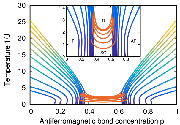
FIG. 3. Constant dimensionality d cross sections of the global phase diagram in Fig. 2. The cross sections are, starting from high temperature, for d = 3, 2.9, 2.8, 2.7, \dots, 2.1, 2 . It is seen that, as the dimensionality d approaches d_c = 2.431 from above, the spin-glass phase disappears at zero temperature.
