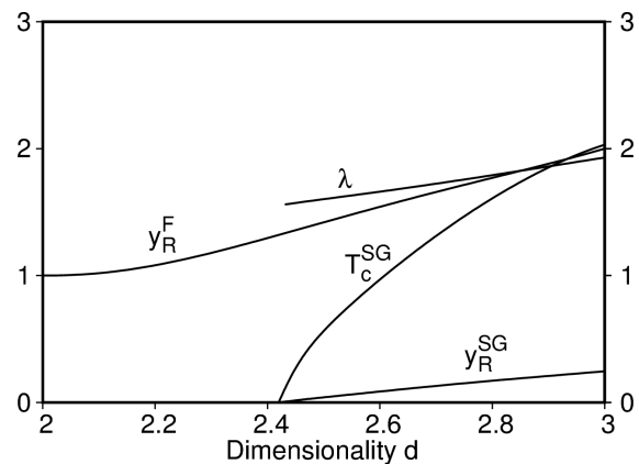
FIG. 6. Spin-glass critical temperature T_c^{SG} at p = 0.5 , spin-glass chaos Lyapunov exponent \lambda , spin-glass-phase runaway exponent y_R^{SG} and ferromagnetic-phase runaway exponent y_R^F , as a function of dimension d . Note that the ferromagnetic phase runaway exponent y_R^F correctly tracks d - 1 .
