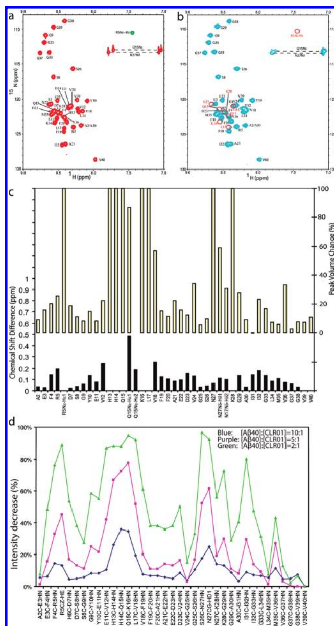
Figure 8. CLR01 binding sites on A\beta determined by solution-state 2D-NMR. (a) ^{15}\text{N}-^1\text{H} spectrum of A\beta_{40} alone (red or green). (b) ^{15}\text{N}-^1\text{H} spectrum of A\beta_{40} in the presence of 30 \mu\text{M} CLR01 (cyan). Red circles indicate resonances that disappeared completely upon addition of CLR01. (c) Resonance perturbation upon addition of 30 \mu\text{M} CLR01 to 60 \mu\text{M} A\beta_{40} . (d) A\beta_{40} /CLR01 mixtures were analyzed by 2D solution-state H(N)CO NMR experiments. A\beta_{40} concentration was kept constant at 60 \mu\text{M} and CLR01 concentration was increased from 6 to 30 \mu\text{M} .
