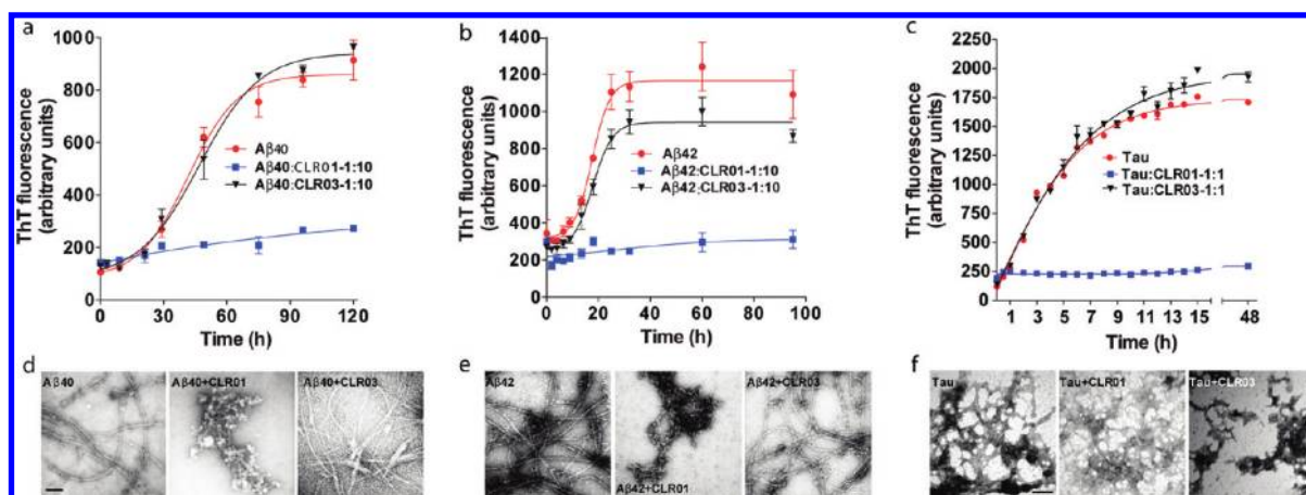
Figure 2. CLR01 inhibits A\beta and tau aggregation. The effect of MTs on \beta -sheet formation by (a) A\beta_{40} , (b) A\beta_{42} , and (c) embryonic tau was assessed by measuring ThT fluorescence. The data are presented as mean \pm SEM of three independent experiments. Morphological analysis of (d) A\beta_{40} , (e) A\beta_{42} , and (f) tau in the absence or presence of MTs was examined at the end of each aggregation reaction. Scale bars indicate 100 nm.
