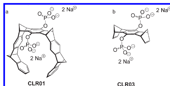
Figure 1. Molecular structures of MTs: (a) CLR01; (b) CLR03. These compounds are slightly basic in aqueous solution and the phosphate groups are partially protonated at pH 7.4.
