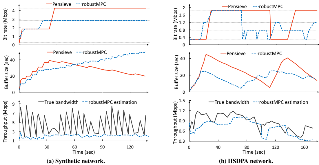
Figure 3: Profiling bitrate selections, buffer occupancy, and throughput estimates with robustMPC [50] and Pensieve.
