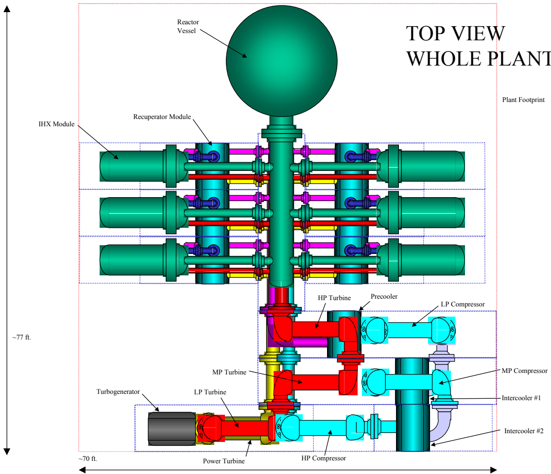
Figure 4: Top Down View of Pebble Bed Reactor Plant
