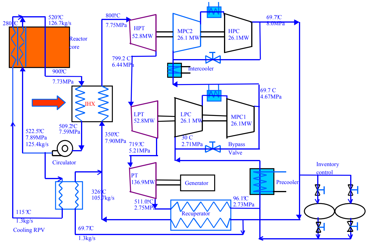
Figure 1: Current Plant Schematic
