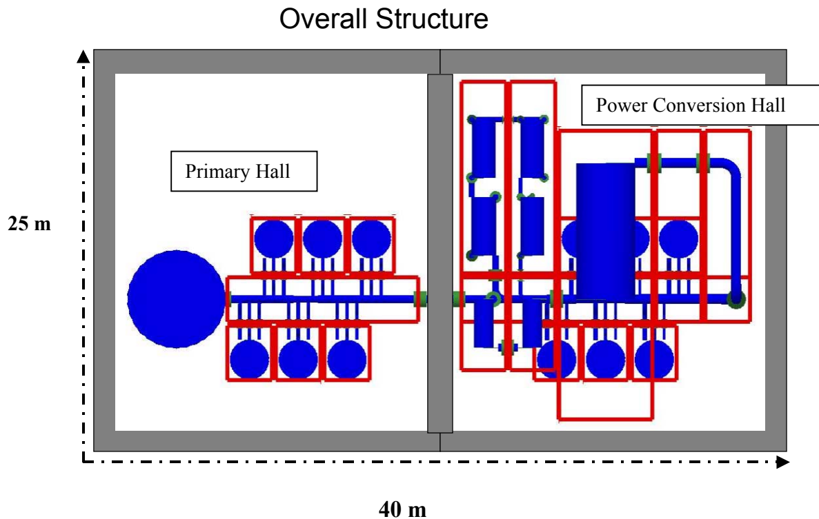
Figure 10: Overall Plant Structural Layout
