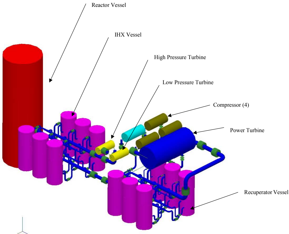
Figure 7: Latest Design Layout to Accommodate Thermal Expansion
