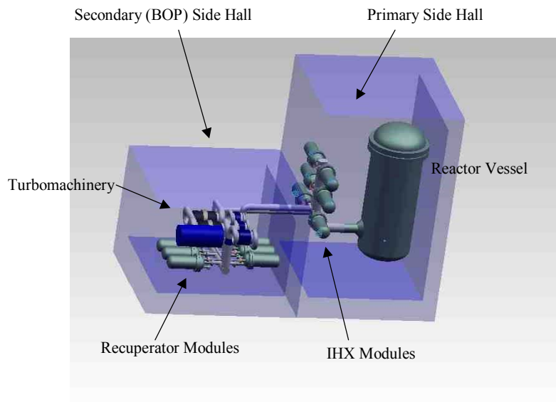
Figure 1: Current Plant Schematic
