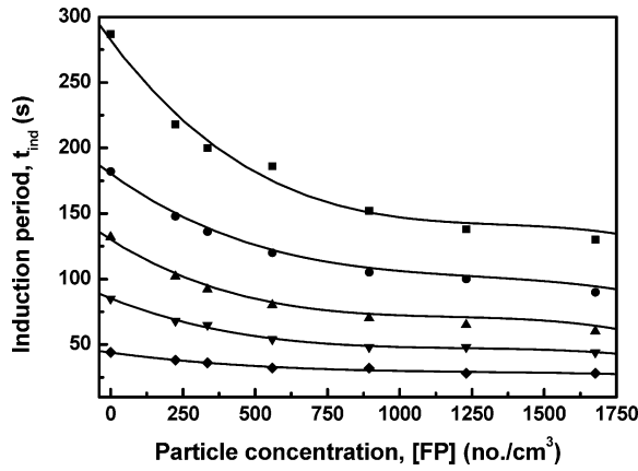
Figure 2. Induction period as a function of the concentration of foreign particles at five different levels of supersaturation: (■) S_a = 4.59 ; (●) S_a = 5.49 ; (▲) S_a = 5.85 ; (▼) S_a = 6.41 ; (◆) S_a = 6.90 .
