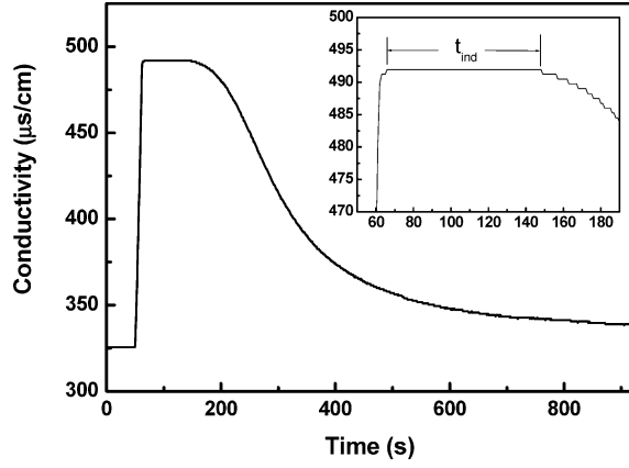
Figure 1. A typical desupersaturation curve for the mixing of 0.0020 M \text{CaCl}_2 and \text{Na}_2\text{CO}_3 solution with 2 mg of diatomaceous earth as the foreign particle at 298 K. The induction period can be determined when that portion of the desupersaturation curve is enlarged, as shown in the upper right corner.
