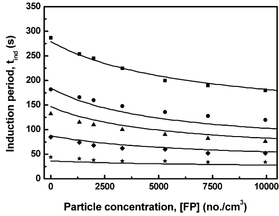
Figure 8. Calculated curves of the induction period calculated by using eq 25 for zirconium oxide as the foreign particle: (■) experimental points for S_a = 4.59 ; (●) experimental points for S_a = 5.49 ; (▲), experimental points for S_a = 5.85 ; (◆) experimental points for S_a = 6.41 ; (★) experimental points for S_a = 6.90 .
