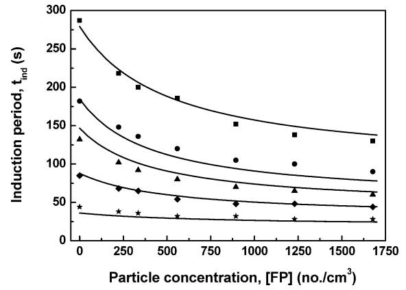
Figure 7. Calculated curves of induction period calculated by using eq 24 for diatomaceous earth as the foreign particle: (■) experimental points for S_a = 4.59 ; (●) experimental points for S_a = 5.49 ; (▲) experimental points for S_a = 5.85 ; (◆) experimental points for S_a = 6.41 ; (★) experimental points for S_a = 6.90 .
