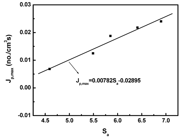
Figure 4. J_{p,\max} as a linear function of S_a for diatomaceous earth as the foreign particle: (■) calculated points ( J_{p,\max} , S_a ).
