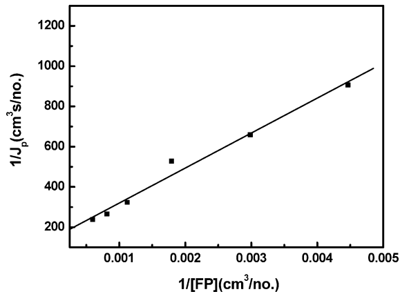
Figure 3. Plot of 1/J_p versus 1/[FP] for the foreign particles of diatomaceous earth at S_a = 4.59 .
