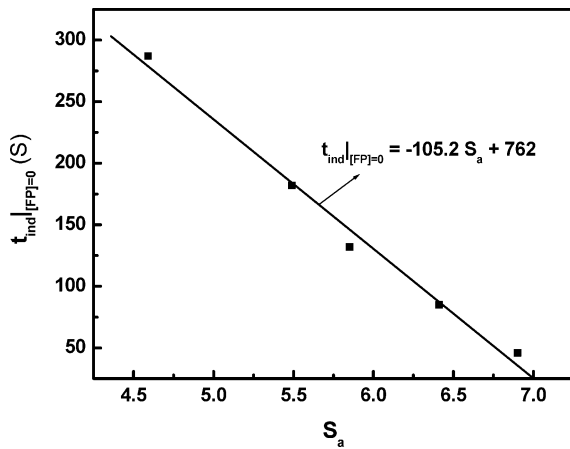
Figure 6. Induction period without adding foreign particles as a linear function of S_a : (■) experimental points.
