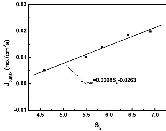
Figure 5. J_{p,max} as a linear function of S_a for zirconium oxide as the foreign particle: (■) calculated points ( J_{p,max} , S_a ).
