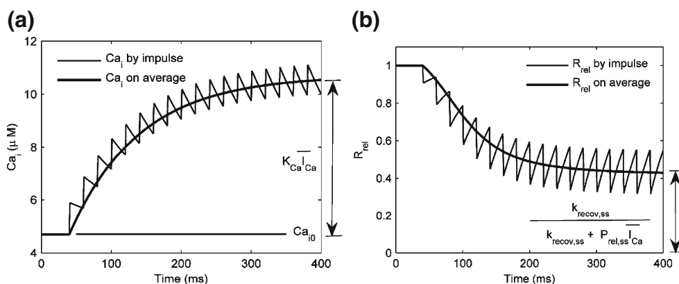
Fig. 2 The instantaneous time courses of key biophysical variables caused by impulses (zig-zag lines). Also the average time courses are represented by the smooth curves. (a) An example of intracellular calcium concentration ( Ca_i ) time course. (b) An example of releasable vesicle ration ( R_{rel} ) time course
