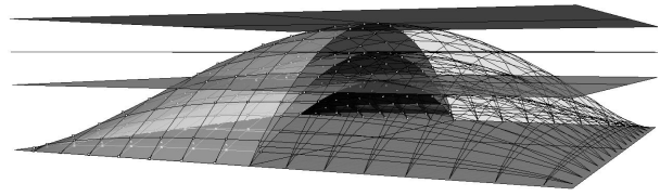
Figure 4. Decreasing the scale factor \zeta of the dual grid means overall lower horizontal forces in the system and hence a deeper solution for the same set of applied loads.
