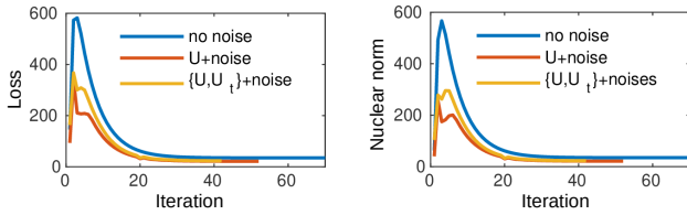
Figure 3: Convergence of LrSTR on Burgers' equation with no noise, U +sparse noise, and \{U, U_t\} +sparse noise. Left is the loss, and right is the nuclear norm of \mathcal{D}(Z, Q)\bar{\xi} .
