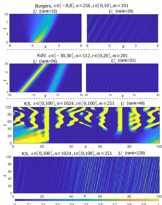
Figure 1: Low-rank numerical solutions U \in \mathbb{C}^{n \times m} and their partial derivatives U_t \in \mathbb{C}^{n \times m} of PDEs (e.g., Burgers, Korteweg-de Vries (KdV) and Kuramoto-Sivashinsky (KS)). U and U_t are collected from all the spatial time series data u(x, t) and u_t(x, t) in the intervals [a, b] and [c, d] with n spatial locations and m time points.
