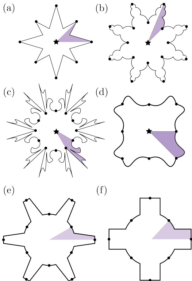
Fig. 6 Example of some irregular shapes that may be constructed from sector reflections of a primitive shape (shaded in purple) for cases of: (a) N = 8 ; (b) N = 16 ; (c) N = 12 ; (d) N = 8 ; (e) N = 12 ; and (f) N = 8 . Panels (e) and (f) demonstrate that gear-like configurations satisfy the conditions of Theorem 2.
