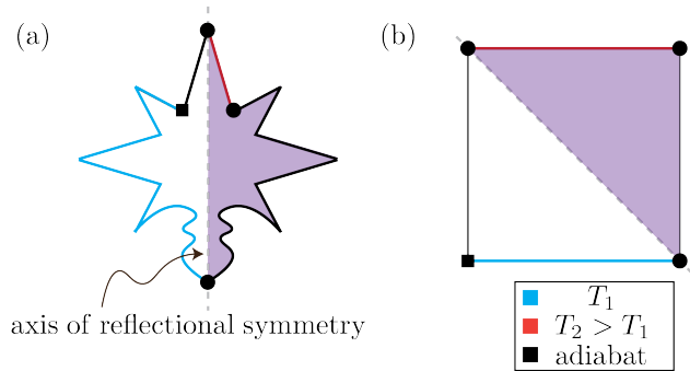
Fig. 7 Conformal equivalence of Yin-Yangs and the square problem with S = 1 . The domain in panel (a) embodies the Yin-Yang symmetry as described in §4.6. By the Riemann mapping theorem, there exists a mapping between the purple shaded section of the domain in (a) and the half-square with the drawn boundary correspondence as drawn in panel (b). The Schwarz reflection principle then gives the remainder of the map (white region with the illustrated boundary correspondence). Since the shape factor of (b) is trivially equal to unity, by the conformal invariance of the shape factor, S = 1 in (a) as well.
