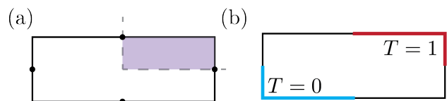
Fig. 4 (a) The rectangle can be constructed by successive reflections of a smaller primitive rectangle (shaded in purple), and N = 4 . (b) An example shape factor problem where S_i = S_e is guaranteed by Theorem 2.
