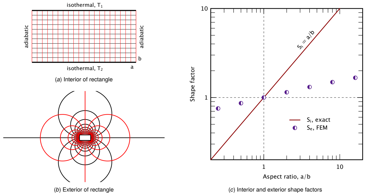
Fig. 1 Interior and exterior shape factor for a rectangle of aspect ratio a/b . The interior shape factor is exactly a/b . The exterior values are from FEM calculations (see Appendix A). The interior and exterior shape factors are equal only for the case of a square ( a = b ) but unequal for rectangles with a \neq b .
