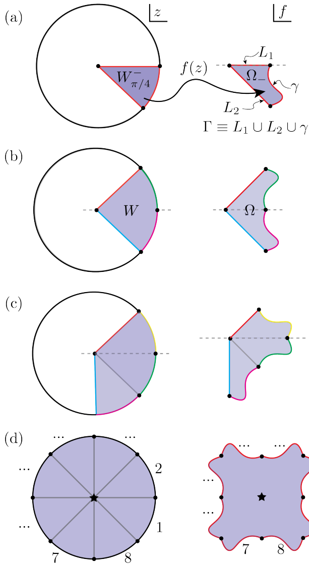
Fig. 2 Demonstration of the sector reflection principle of Herisch [8]. The Riemann mapping theorem guarantees the existence of an analytic mapping f(z) between W_{\pi/4}^- and \Omega_- as indicated in panel (a). The Schwarz reflection principle guarantees f(z) may be analytically extended to W with the boundary correspondence as indicated in panel (b). Rotating clockwise by \pi/4 and reflecting again leads to panel (c). By performing rotations and reflections, the domain of analyticity of f(z) may be extended to the entire unit circle. The image and boundary correspondence of the mapping from the unit circle is given in panel (d).
