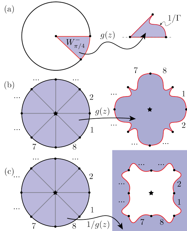
Fig. 3 Construction of the map between the unit circle interior and the exterior problem, using sector reflections. The Riemann mapping theorem guarantees a mapping g(z) between W_{\pi/4}^- and the region enclosed by 1/\Gamma , as depicted in (a). By applying sector reflections (as was done in Fig. 2) the domain of analyticity of g(z) is extended to the entire unit disc as illustrated in panel (b). Note that the map in panel (b) is to an entirely new shape. The map 1/g(z) then sends the interior of the unit circle to exterior domain of interest.
