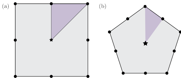
Fig. 5 Example primitive sectors for the (a) square ( N = 8 ) and (b) pentagon ( N = 10 ) are shaded in purple. The conformal map from the interior of the unit disk to the square maps each wedge spanning 2\pi/N to each of the primitive shapes in Fig. 5.
