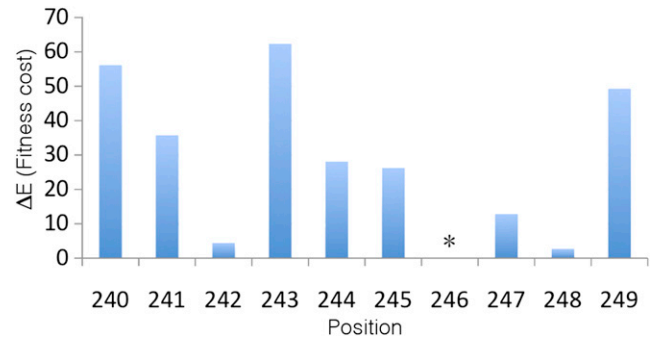
Figure 4. Escape Mutations Associated with HLA B*57 in the TW10 (Gag 240–249 ) Epitope Occur at Residues Predicted to Incur the Smallest Fitness Penalty
