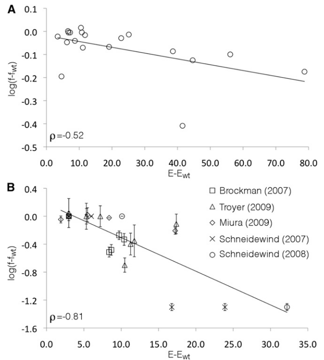
Figure 2. Comparison of Our Theoretical Metric of Fitness ( E ) and Experimental In Vitro Replicative Fitness Data
