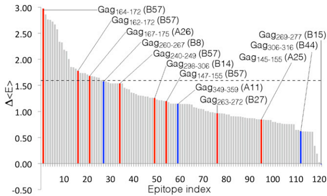
Figure 6. Fitness Costs Associated with Targeting Different HLA-Associated Immunodominant Epitopes
