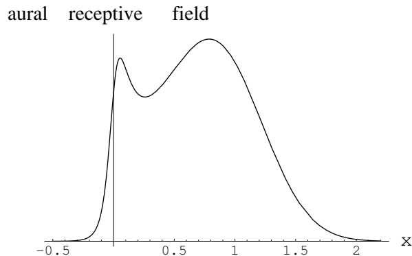
FIG. 1 An aural receptive with two peaks, obtained from Eq. (22) for l = 0.5 , L = 0.1 , and c = 1.1 .
