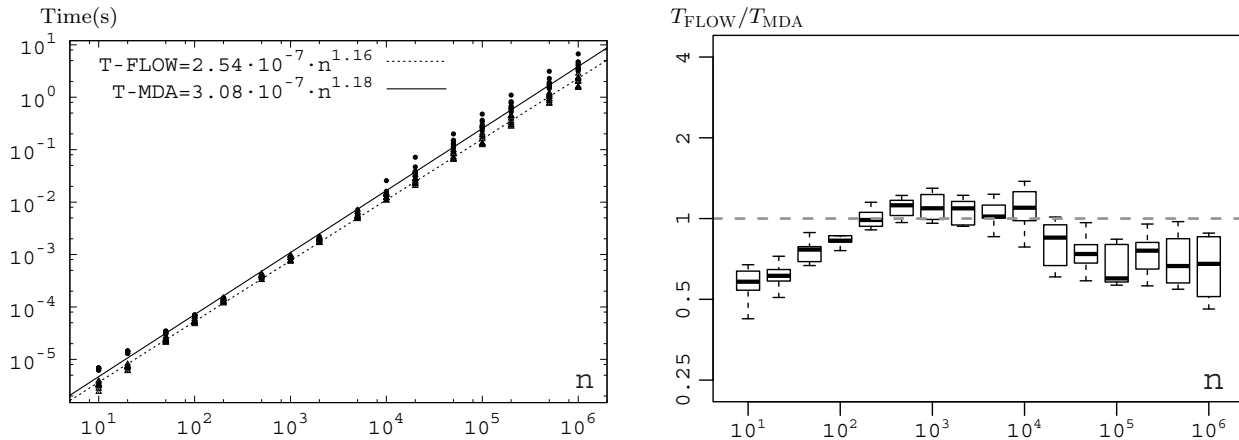
Figure 1: Varying n \in \{10, \dots, 10^6\} and m = n . Left figure: CPU time of both methods as n and m grow. Right figure: Boxplots of the ratio T_{\text{FLOW}}/T_{\text{MDA}} .
