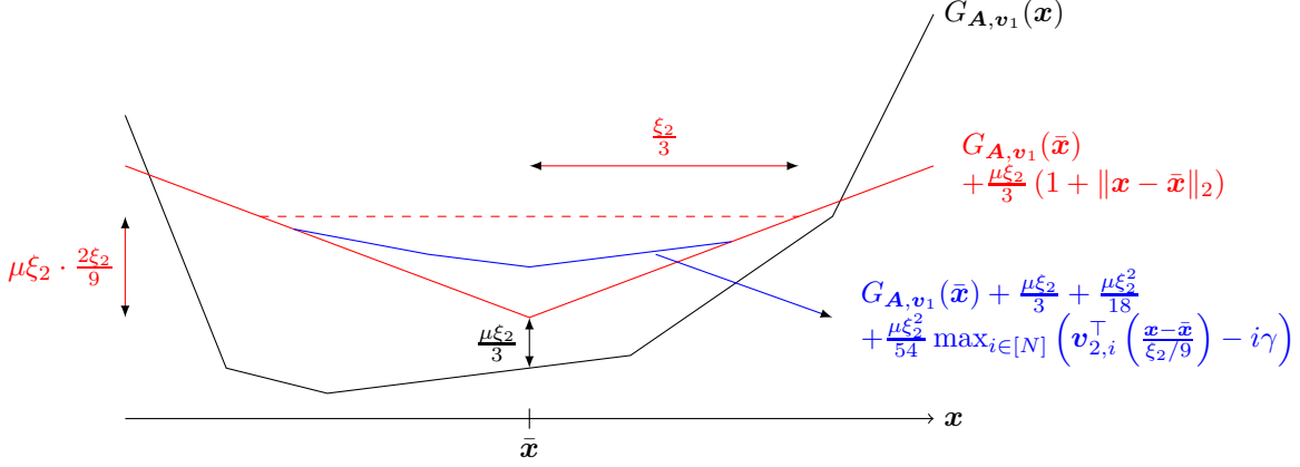
Figure 3: Representation of the procedure to rescale the optimization function.
