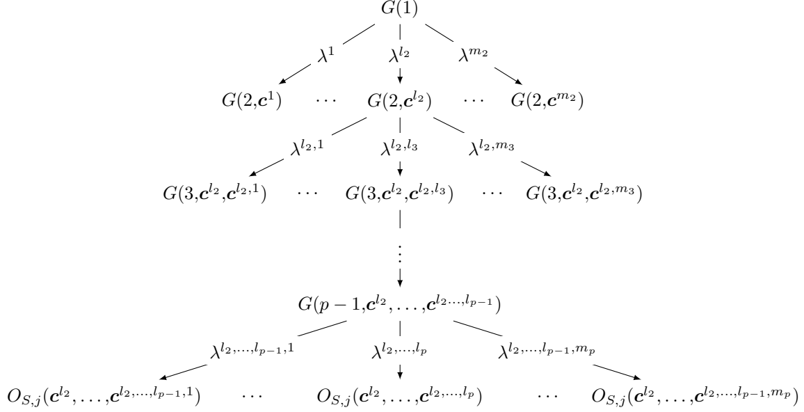
Figure 2: Computation tree representing the recursive calls to ApproxOracle starting from the calls to ApproxOracle(1, 1, ·) from Algorithm 4
