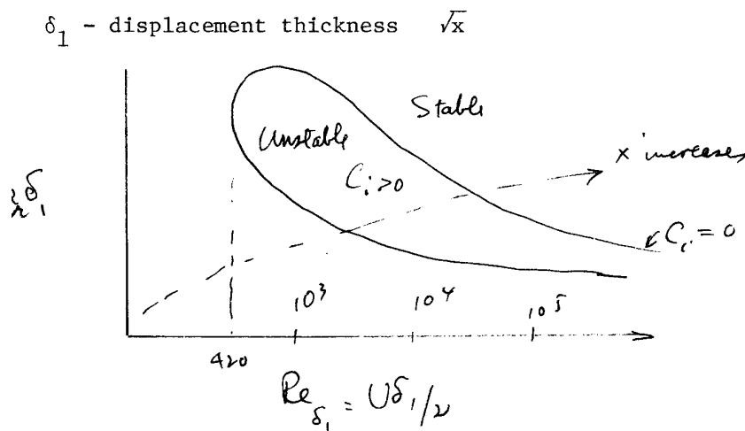
Figure 5.4.2: Instability region of a Blasius boundary layer. k_r\delta_1 vs. Re_{\delta_1} where \delta_1 is the displacement thickness which increases with \sqrt{x} .
