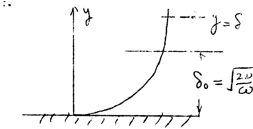
Figure 5.4.1: An oscillatory Stokes boundary layer
