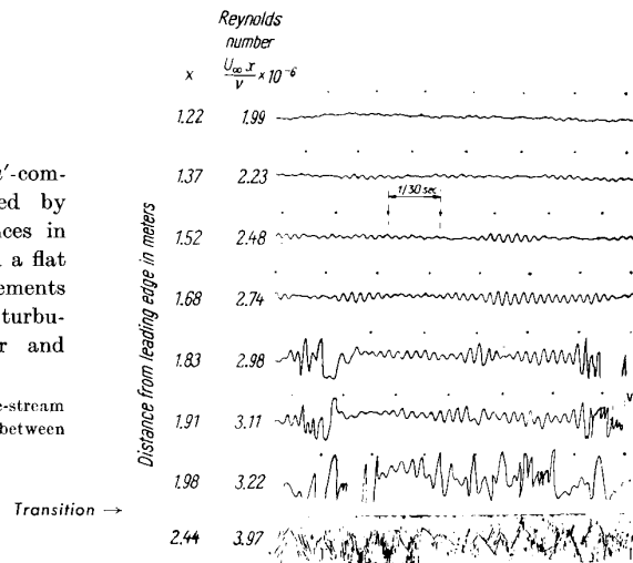
Figure 5.4.4: Experiments on boundary layer instability. From Schlichting.
