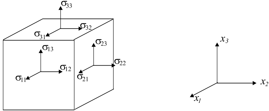
Figure 1.4.1: Stress components on a fluid element
