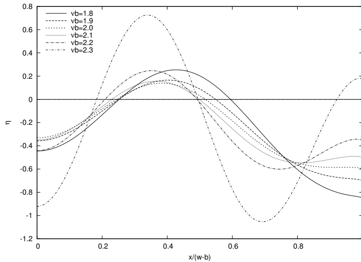
Figure 17. Evolution of moonpool wave elevation \text{Re } \eta(x) from \nu b = 1.8 to 2.3.
