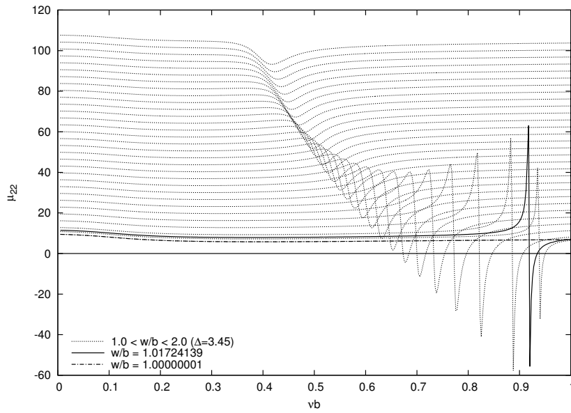
Figure 9. Plot of \mu_{22} versus \nu b for small moonpools, with w/b = [1.0(0.0345)2.0] , d/b = 1.0 , h/d = 20.0 .
