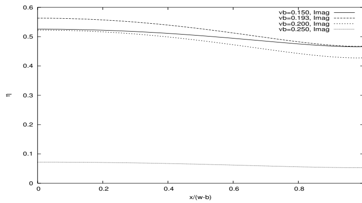
Figure 12. Free surface elevation, \text{Im } \eta(x) in moonpool, from \nu b = 0.15 to 0.25 , w/b = 5.0 .
