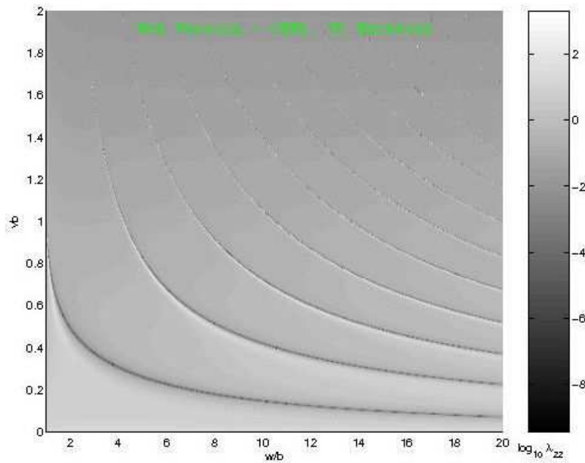
Figure 8. Contours of \lambda_{22} with w/b and \nu b as variables, b/d = 1 , h/d = 20 .
