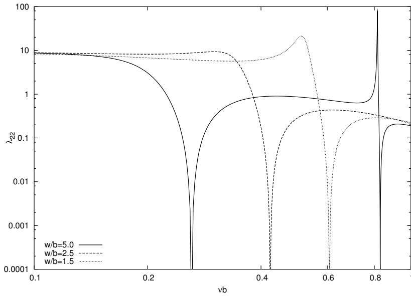
Figure 6. Zero damping property for three moonpool widths: w/b = 5.0, 2.5, 1.5 .
