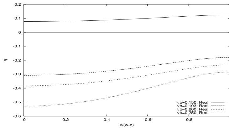
Figure 11. Free surface elevation, \text{Re } \eta(x) in moonpool, from \nu b = 0.15 to 0.25 , w/b = 5.0 .
