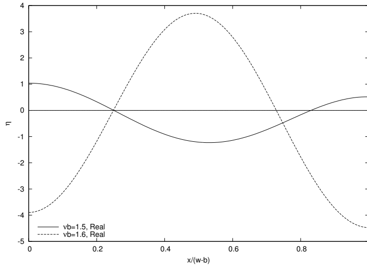
Figure 16. Free surface elevation, \text{Re } \eta(x) , as frequency crosses the second resonance near (\nu b)_2 .
