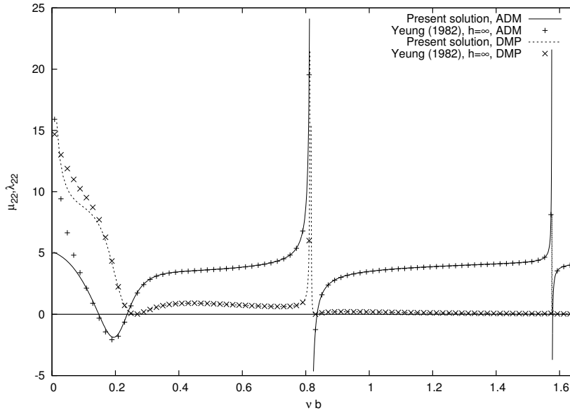
Figure 2. Heave hydrodynamic coefficients for twin cylinders, b/d = 1.0 , w/b = 5.0 , h/d = 20 .
