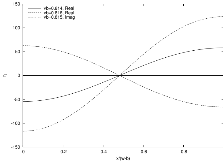
Figure 14. Change in \eta(x) across the first resonance frequency, (\nu b)_1 .
