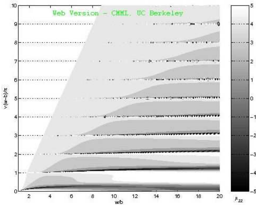
Figure 10. Contours of \mu_{22} plotted against w/b and \nu(w-b)/\pi .
