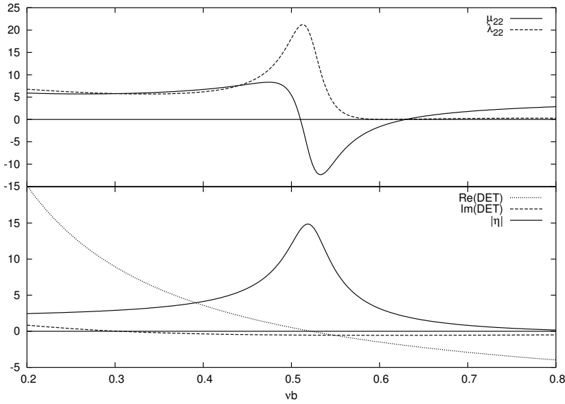
Figure 5. Heave hydrodynamic coefficients at the Helmholtz resonance, shown with determinant of (43) and (44) and wave elevation averaged over moonpool |\bar{\eta}| , b/d = 1.0 , w/b = 1.5 .
