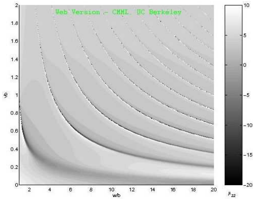
Figure 7. Contours of \mu_{22} with w/b and \nu b as variables, b/d = 1 , h/d = 20 .
