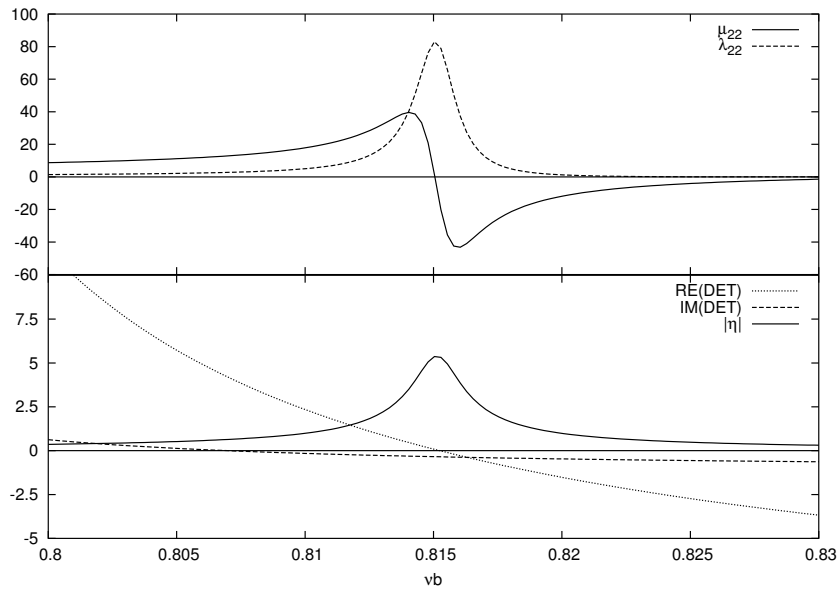
Figure 4. Heave hydrodynamic coefficients at the first-order resonance, shown with determinant of (43) and (44) and wave elevation averaged over moonpool |\bar{\eta}| , b/d = 1.0 , w/b = 5.0 .
