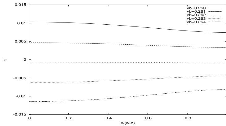
Figure 13. Free surface elevation, \text{Im } \eta(x) in moonpool, across (\nu b)_o = 0.2617 .
