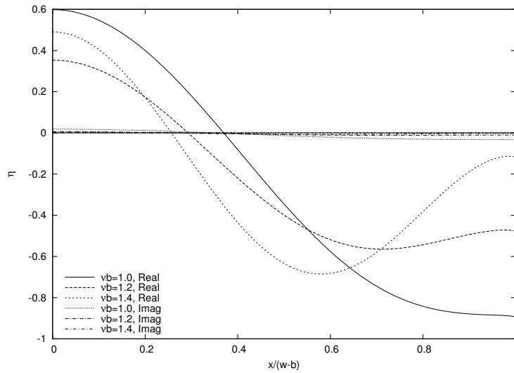
Figure 15. Evolution of moonpool free-surface profile, \eta(x) , from \nu b = 1.0 to 1.4.
