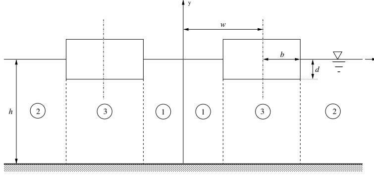
Figure 1. Schematic of the fluid domain.
