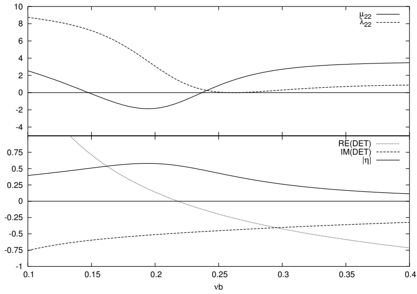
Figure 3. Heave hydrodynamic coefficients at the Helmholtz resonance, shown with determinant of (43) and (44) and wave elevation averaged over moonpool |\bar{\eta}| , b/d = 1.0 , w/b = 5.0 .
