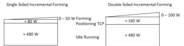
Fig. 3 Results power measurements of SSIF and DSIF
