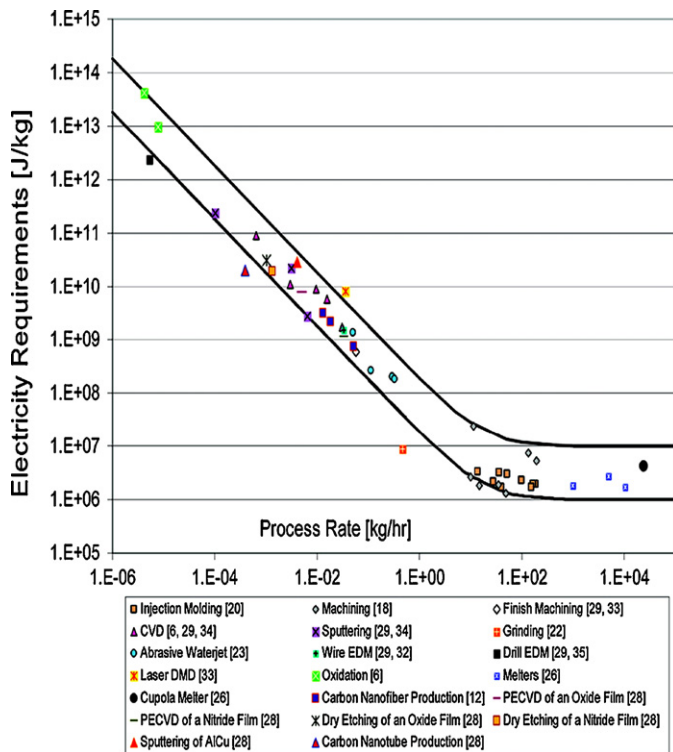
Fig. 3.4. Electricity used per unit of material processed for various manufacturing processes as function of processing rate.
