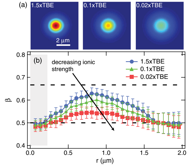
FIG. 4 (color online). (a) Time average intensity distribution, \langle I \rangle , of T4 confined to 1\ \mu\text{m} slits in different ionic strength buffers. Notice, decreasing the ionic strength expands the in-plane size of the DNA coil. (b) Stretched exponential results for the T4 DNA in three different ionic strength buffers; 1.5 (56.9), 0.1 (5.3), and 0.02 \times TBE (1.5 mM).
