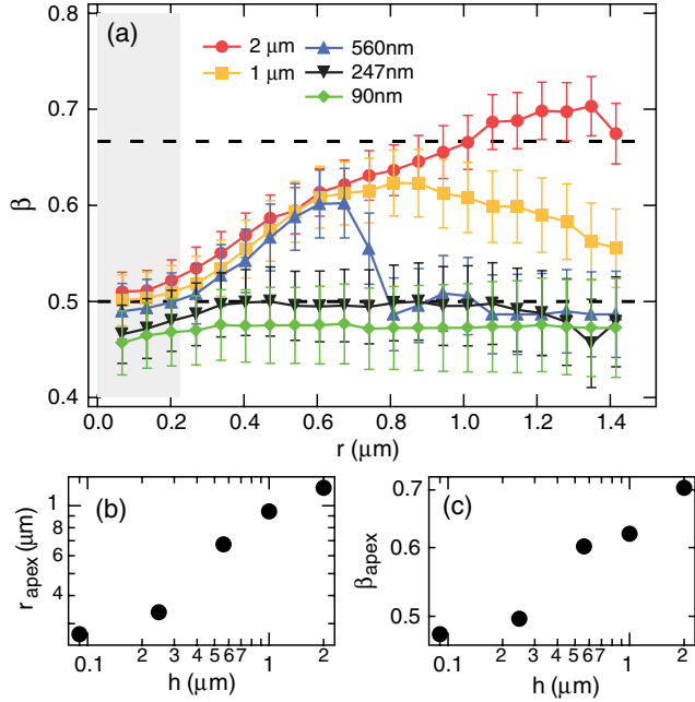
FIG. 2 (color online). (a) Summary of stretching exponent for the time-decay of the dynamic structure factor, S(r, \delta t) for \lambda -DNA at variable channel heights. The horizontal dashed lines indicate Zimm ( \beta = 2/3 ) and Rouse ( \beta = 1/2 ) behavior. The grey shaded area represents the optical resolution limit, r < 220 nm. The lower graphs show the distance (b) r_{\text{apex}} at which the maximum value of (c) \beta_{\text{apex}} is attained for different channel heights.
