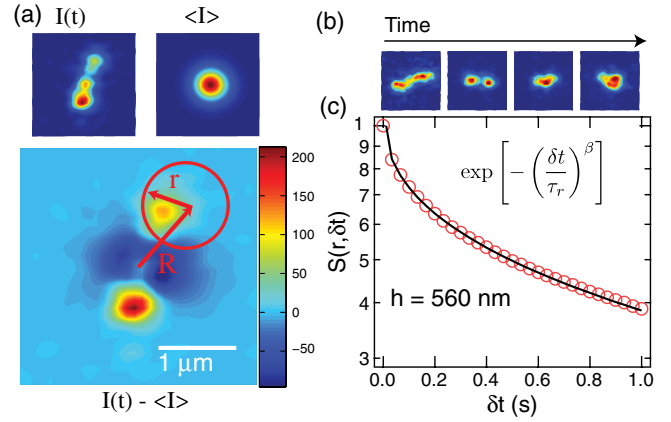
FIG. 1 (color online). Schematic of our analysis method for extracting HI information within \lambda -DNA confined to a 560 nm tall slit channel. (a) Example of an instantaneous 2D image with intensity I(t) , the time average of all images \langle I \rangle and visual representation of the instantaneous intensity perturbation from the average, I(t) - \langle I \rangle . The red arrows represent the position vectors in S(r, \delta t) = \sum_{\theta} \sum_{\mathbf{R}} C(\mathbf{R}, \mathbf{R} + \mathbf{r}, \delta t) and the circle indicates the continuous integration over all \theta . The analysis is done for all time-varying images such as those in (b). Afterwards, we perform a nonlinear regression with a stretched exponential S(r, \delta t) \propto \exp[-(\delta t/\tau_r)^\beta] as shown in (c).
