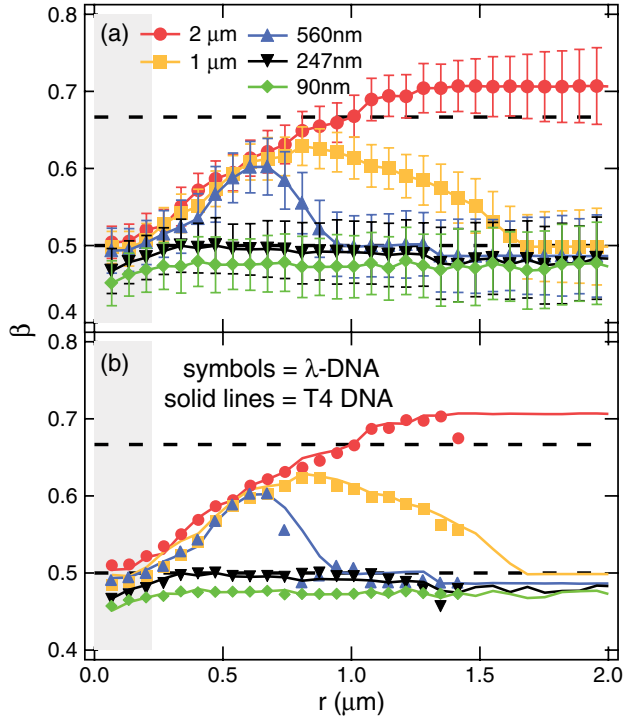
FIG. 3 (color online). (a) Summary of stretching exponent for the time decay of the dynamic structure factor, S(r, \delta t) for T4 DNA at variable channel heights. It is important to compare this data to the \lambda -DNA data as shown in (b). The solid markers are that of \lambda -DNA, and the solid lines are T4 DNA. The T4 DNA data extends further in r because the molecule is larger than \lambda -DNA.
