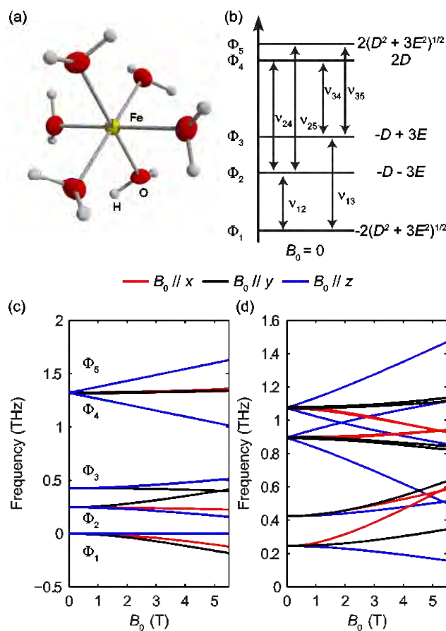
Fig. 11. (a) The structure of \text{Fe}(\text{H}_2\text{O})_6^{2+} . (b) Zero-field magnetic sublevel diagram of the HS Fe(II) in \text{Fe}(\text{H}_2\text{O})_6(\text{BF}_4)_2 ( S = 2 spin system), where a positive D value is assumed. The magnetic dipole-allowed transitions are shown by the arrows. (c) Zeeman splitting of the magnetic sublevels as a function of B_0 . (d) Frequencies of magnetic dipole-allowed transitions as functions of the external magnetic field. In (c) and (d), the color coding indicates the direction of B_0 with respect to the molecular axes, as shown by the legend.
