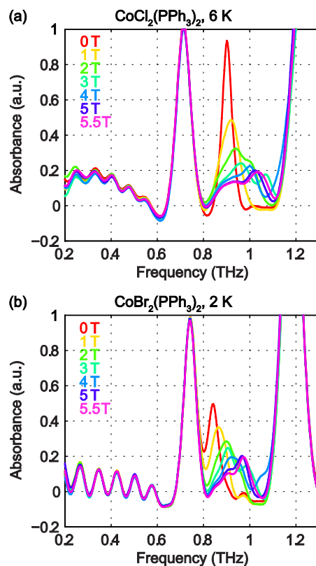
Fig. 9. Field-dependent absorbance spectra of \text{CoCl}_2(\text{PPh}_3)_2 at 6 K (a) and \text{CoBr}_2(\text{PPh}_3)_2 at 2 K (b). The spectral modulations are artifacts of Fourier transformation. The spectra are color-coded based on the values of B_0 shown in the legends.
