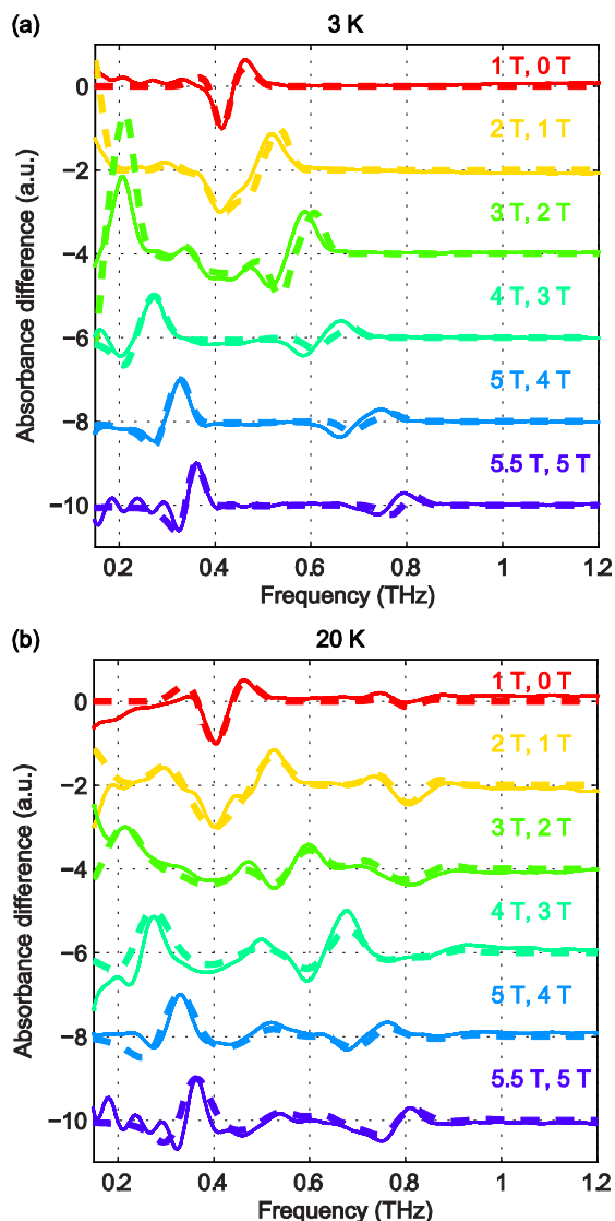
Fig. 6. Experimental difference absorbance spectra (solid lines) and simulated difference intensity spectra (dashed lines) at 3 K (a) and 20 K (b) at various B_0 levels. The spectra are color-coded according to the values of B_0 indicated in the figure.
