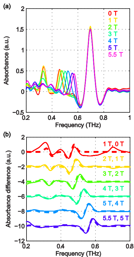
Fig. 16. (a) Field-dependent absorbance spectra of \text{NiCl}_2(\text{PPh}_3)_2 at 2 K. The two spin resonance peaks show splittings and shifts as a function of B_0 . The strong absorption peak is likely due to lattice vibrations. (b) Experimental difference absorbance spectra (solid lines) and simulated difference intensity spectra (dashed lines) for \text{NiCl}_2(\text{PPh}_3)_2 at 2 K. The spectra are color-coded according to the values of B_0 indicated in each figure.
