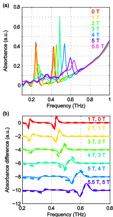
Fig. 13. (a) Field-dependent absorbance spectra of \text{Fe}(\text{H}_2\text{O})_6(\text{BF}_4)_2 at 1.8 K. The two spin resonance peaks show splittings and shifts as a function of the applied magnetic field. (b) Experimental difference absorbance spectra (solid lines) and simulated difference intensity spectra (dashed lines) for \text{Fe}(\text{H}_2\text{O})_6(\text{BF}_4)_2 at 1.8 K. The spectra are color-coded according to the magnetic field values indicated in each figure.
