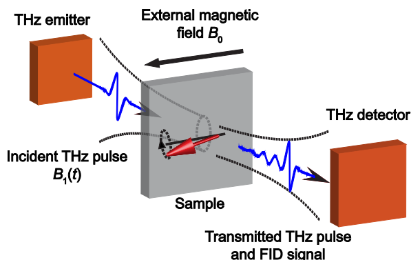
Fig. 1. Schematic illustration of experimental geometry. Single-cycle THz pulses are generated by illuminating the THz emitter with fs laser pulses. The THz pulses are incident onto the sample to excite the spin transitions. The transmitted THz pulses and FID signals are directed into the THz detector. Fs laser pulses are overlapped with the THz fields at the THz detector for phase-resolved detection of the THz signals. The sample is placed in a cryostat with an external magnetic field B_0 perpendicular to the THz magnetic field B_1 (e.g. the Voigt geometry shown here). Fourier transformation of the THz signals yields the EPR spectra. In this work, the THz emitter and detector are both ZnTe crystals as described in the Supplementary Information.
