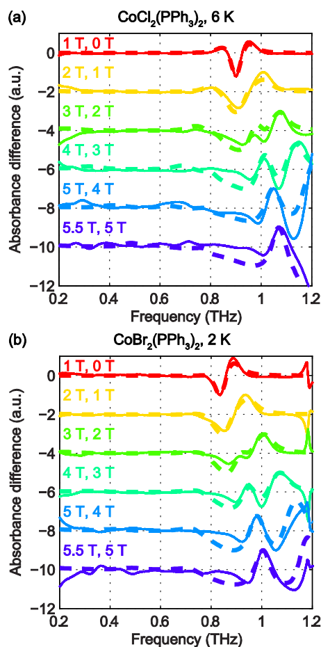
Fig. 10. Experimental difference absorbance spectra (solid lines) and simulated difference absorbance spectra (dashed lines) for \text{CoCl}_2(\text{PPh}_3)_2 at 6 K (a) and \text{CoBr}_2(\text{PPh}_3)_2 at 2 K (b). The spectra are color-coded according to the values of B_0 indicated in the figure. Additional features around 1.2 THz in (b) are due to the strong nearby vibrational absorption peak in each compound.
