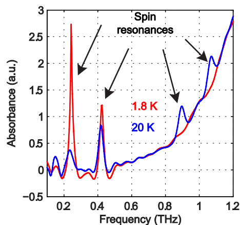
Fig. 12. Zero-field absorbance spectra of \text{Fe}(\text{H}_2\text{O})_6(\text{BF}_4)_2 at 1.8 K (red) and 20 K (blue). At 1.8 K, two strong peaks are assigned as the spin resonances resulting from two transitions. At 20 K, four peaks are assigned as the spin resonances resulting from six transitions. In this case the peak frequencies could be determined accurately without subtraction of the background absorbance.
