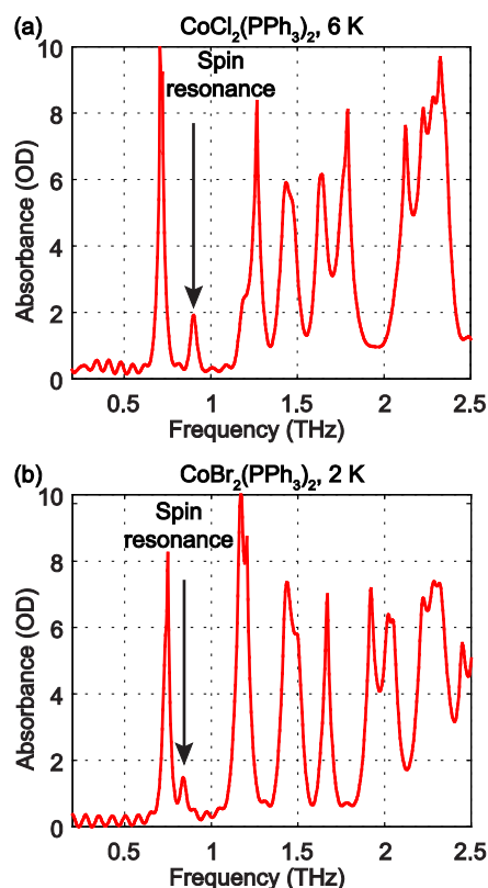
Fig. 8. Zero-field absorbance spectra of \text{CoCl}_2(\text{PPh}_3)_2 at 6 K (a) and \text{CoBr}_2(\text{PPh}_3)_2 at 2 K. The spin resonance peak in each figure is indicated by the arrow. Other strong absorption peaks are due to vibrations.
