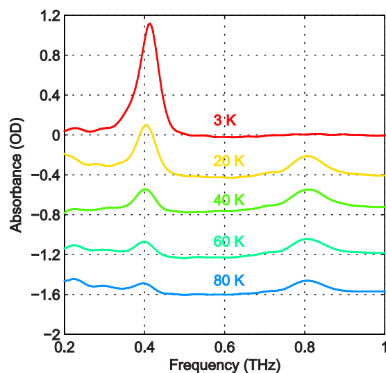
Fig. 4. Temperature-dependent zero-field absorbance spectra of hemin after background subtraction. The data are color-coded according to the temperatures. The higher-frequency peak disappears and the lower-frequency peak shifts slightly at reduced temperatures.
