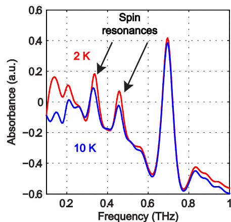
Fig. 15. Zero-field absorbance spectra of \text{NiCl}_2(\text{PPh}_3)_2 at 2 K (red) and 10 K (blue). The two spin resonance peaks are shown by the arrows and are present at both temperatures. The stronger peak is due to a vibration.
