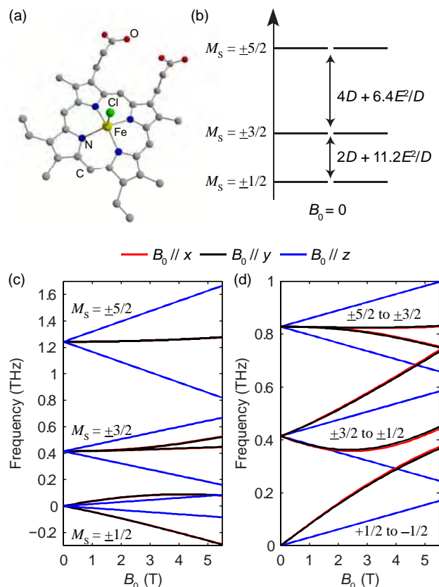
Fig. 2. (a) The structure of hemin. Hydrogen atoms are omitted for clarity. (b) Zero-field magnetic sublevel energy diagram of the HS Fe(III) in hemin ( S = 5/2 spin system), where a positive D value is assumed. The magnetic dipole-allowed transitions are shown by the double arrows. (c) Calculated Zeeman splitting of the magnetic sublevels as a function of B_0 in hemin. (d) Calculated frequencies of magnetic dipole-allowed transitions as functions of B_0 in hemin. In (c) and (d), the color coding indicates the direction of B_0 with respect to the molecular axes as shown by the legend. The black and red curves ( B_0 // x and y ) are too closely overlapped to distinguish in these plots.
