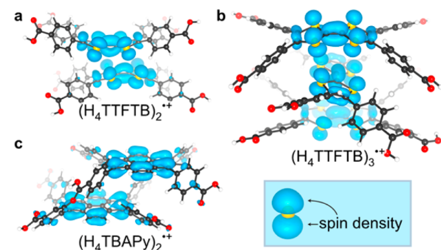
Figure 3. The calculated spin densities ( \rho_{\uparrow} - \rho_{\downarrow} ) of (a) (\text{H}_4\text{TTFTB})_2^{\bullet+} and (b) (\text{H}_4\text{TTFTB})_3^{\bullet+} showing full hole delocalization across the TTF core. (c) The one-electron-oxidized (\text{H}_4\text{TBAPy})_2^{\bullet+} shows similar spin delocalization across the conjugated pyrene core.
