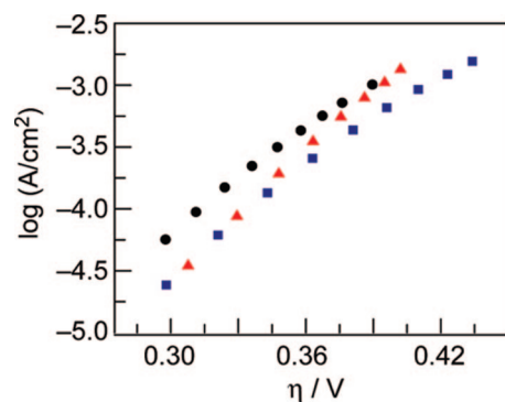
Figure 5. Tafel plot, \eta = (V_{\text{appl}} - IR - E^{\circ}) , of a catalyst film deposited from and operated in 0.1 M Pi electrolyte, pH 7.0 (●), 0.1 M MePi electrolyte, pH 8.0 (■), and 0.1 M Bi electrolyte, pH 9.2 (▲).
