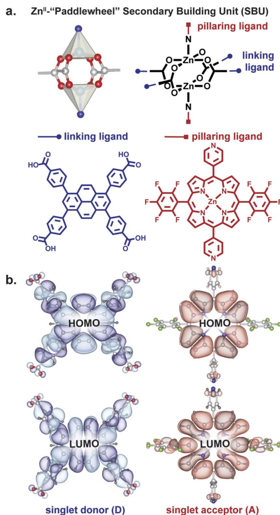
Fig. 2 (a) Building blocks of the paddlewheel pillared PyP-MOF. Rectangular 4,4',4''',4''''-(pyrene-1,3,6,8-tetrayl)tetrabenzoic acid forms two-dimensional grids, which are connected by porphyrin-based pillaring ligands into a three-dimensional network. (b) Frontier orbitals calculated for the donor and acceptor moieties.
