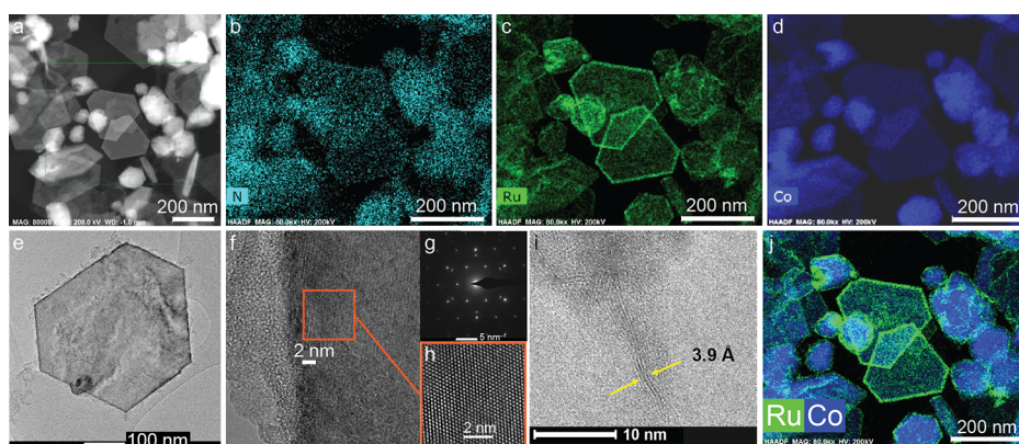
Figure 5. STEM image (a), TEM images (e, f, h, i), fast Fourier transform (g), and EDS mapping for N (b), Ru (c), and Co (d, j) of RuCo formed in butanol-upgrading reactions with 1 in the presence of 5 mol % NaOBU.
