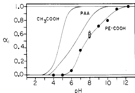
Figure 13. Extent of ionization \alpha_i (eq 3) obtained for PE-CO 2 H as a function of pH using ATR-IR spectroscopy. The experimental points are taken from the types of experiments summarized in Figure 12 using eq 8 and 9. The crosshatched oval at pH 8 contains the data points determined by using seven buffers (0.01 M). 45 Other curves shown are for acetic acid 43 and polyacrylic acid (PAA). 44
