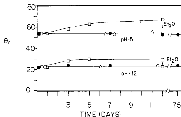
Figure 5. Variation of contact angle (using water at pH 5 and 12) of PE-CO 2 H with time of storage under different conditions. Films were not previously annealed; T = 20^\circ\text{C} . Storage conditions: (●) under dry argon; (○) under argon saturated with water vapor; (△) under water; (□) exposed to laboratory atmosphere. Note that rinsing with ether removed the hydrophobic contaminants adsorbed on the surface of the films.
