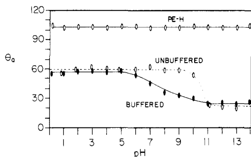
Figure 1. Dependence of advancing contact angle ( \theta_a ) of buffered (●) and unbuffered (○) aqueous solutions on PE-CO 2 H. Unoxidized polyethylene (PE-H) is shown as a control. The buffer used was 0.10 M phosphate.
