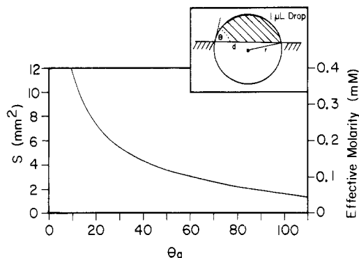
Figure 3. Surface area (idealized planar area, \text{mm}^2 ) and effective concentration of surface groups (mM) under a 1- \mu L drop, for various values of \theta_a , calculated using eq 7. The construction used to arrive at eq 7 is shown at the top of the figure. The shape of the drop is assumed to be a portion of a sphere of radius r . The density of CO 2 H groups is assumed to be 20 \times 10^{14} \text{ cm}^{-2} (that is, the measured density on PE-CO 2 H; for a planar close-packed monolayer, the values of effective molarity given in the figure should be divided by \sim 4 ).
