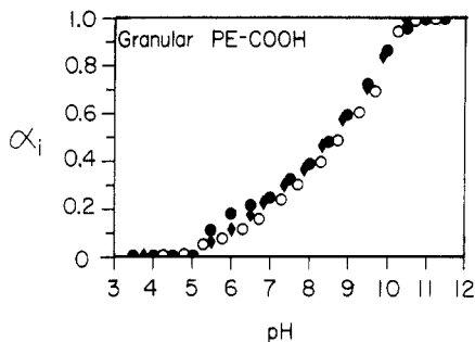
Figure 20. Ionization ( \alpha_i ) determined by direct potentiometric titration as a function of pH for (●) granular PE-CO 2 H, (○) granular PE-CO 2 H derived from hydrolyzed granular PE-CO 2 CH 3 , and (◆) granular PE-CO 2 H in the presence of 0.1 M NaCl.
