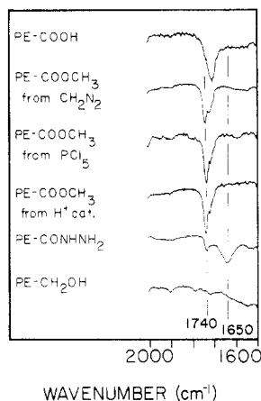
Figure 10. ATR-IR spectra of the carbonyl region of derivatives of PE-COOH.
