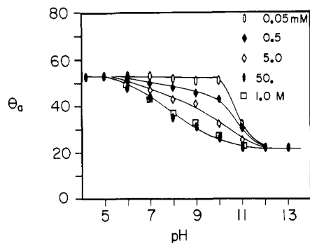
Figure 17. Dependence of \theta_a on pH using different buffer concentrations on PE-CO 2 H. Buffers used are the same as Figure 16 except at 1.0 M where liquid/vapor surface tension changes and ionic strength effects on \theta_a can be significant. At 1.0 M the following buffers were substituted: pH 6 and 7, ethylenediamine; pH 8, Tris; pH 9 and 10, glycine; pH 11, \gamma -aminobutyric acid.
