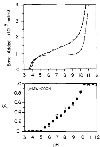
Figure 19. Top: Dependence of pH of UHMW-CO 2 H suspended in water (●) and of water alone (○) as a function of added 0.1 N NaOH. Bottom: Ionization ( \alpha_i ) of UHMW-CO 2 H as a function of pH: (●) determined from the data in the upper part of this figure by eq 10 for UHMW-CO 2 H chips; (○) determined from changes in \theta_a with pH (Figure 15) for UHMW-CO 2 H sheets.
