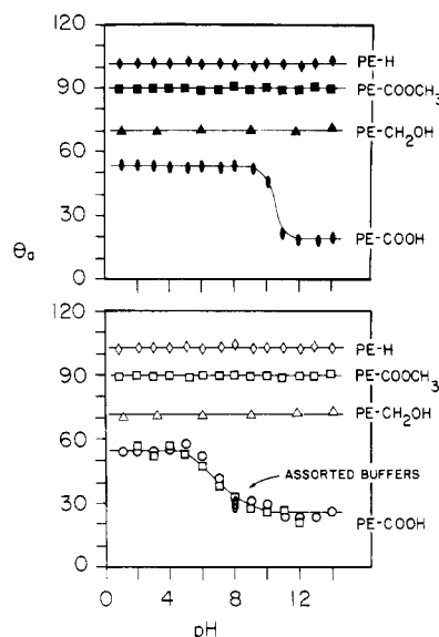
Figure 16. Dependence of \theta_a on pH for surface-functionalized polyethylenes. Top: Using unbuffered aqueous solutions (pH adjusted with NaOH or HCl). Bottom: Using buffered aqueous solutions. 45 Buffers: (□) 0.1 M phosphate buffer; (○) all others (0.05 M), pH 1, 0.1 N HCl; pH 2, maleic acid; pH 3, tartaric acid; pH 4, succinic acid; pH 5, acetic acid; pH 6, maleic acid; pH 7 and 8, HEPES; pH 9 and 10, CHES; pH 11, triethylamine; pH 12, phosphate; pH 13, 0.1 N NaOH. The crosshatched oval labeled "assorted buffers" at pH 8 includes data for phosphate, MOPS, HEPES, TAPS, TRIS, triethanolamine.
