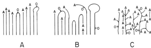
Figure 8. Schematic representations of possible structures of PE-CO 2 H. In each, A = CO 2 H, =O = ketone, and ~ = -(CH 2 ) n -. Each is drawn as if the polyethylene chains entering the oxidized region were crystalline; the argument is not changed if they are amorphous. Model A represents a limit of surface oxidation. The surface is rough, but no acid groups exist in the interior of the polymer. B represents a more plausible model: the groups in contact with water are a mixture of carboxylic acid, ketone, and methylene groups. Oxidized moieties also are found in the sub-surface region. Although two acid groups do not exist on a single short polyethylene chain, a ketone can exist on a chain terminated by an acid group. Model C cannot represent the surface. The oxidation reaction does not introduce oxidized groups as branches, and low molecular weight species would be lost from the material on rinsing with water.
