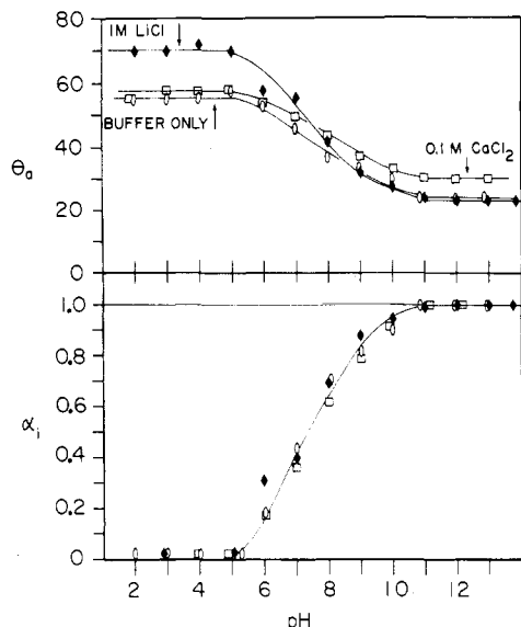
Figure 22. Effects of added salts on \theta_a and \alpha_1 as functions of pH (all systems were buffered with 0.05 M organic buffers). Salts: ( \blacklozenge ) 1 M LiCl; ( \circ ) no added salts; ( \square ) 0.1 M \text{CaCl}_2 .
