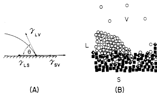
Figure 2. Schematic representations of an ideal (A) and real (B) drop of liquid (L) in contact with solid (S) and vapor (V) with contact angle \theta . The symbols in B represent: (○) water molecules; (Δ) dissolved solutes (phosphate, buffer salts); (◇, ◊) polar surface groups (CO 2 H, CO 2 - , C=O, ...); (■) nonpolar surface groups (CH 2 , CH 3 , ...).
