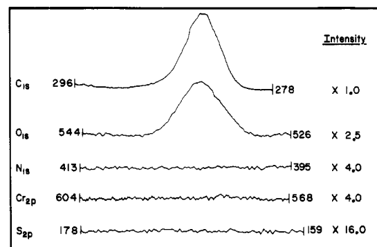
Figure 7. ESCA (XPS) survey spectra of unoxidized and oxidized polyethylene (top left) and the composition of the surface of PE-CO 2 H (top right) determined by integrating the peaks obtained by analyzing only over the binding energies characteristic of elements of interest (bottom). 37
