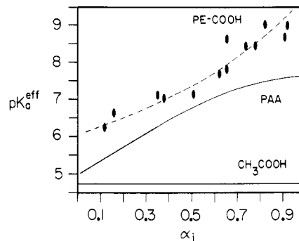
Figure 21. Variation in the effective or apparent pK_a ( pK_a^{\text{eff}} , eq 11) with the extent of ionization. The dashed line represents a visual fit of eq 11 to data of the sort in Figure 18 (●). Curves for poly(acrylic acid) (PAA) 44 and CH 3 CO 2 H 43 are included for comparison.
