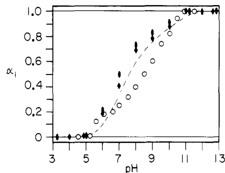
Figure 18. Extent of ionization, \alpha_i , as a function of pH for PE-CO 2 H: (●) phosphate buffer; (◆) organic buffers. The dashed line summarizes the ATR-IR data from Figure 13 for comparison. Data obtained by direct potentiometric titration of granular PE-CO 2 H (○) are also shown.
