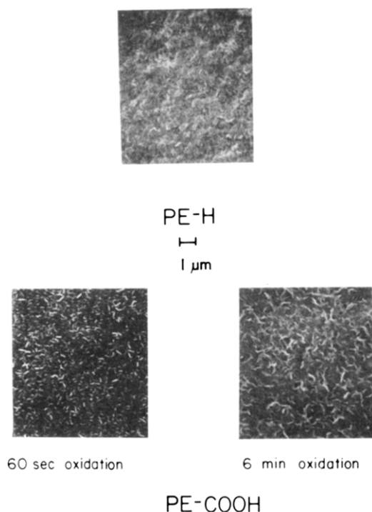
Figure 9. SEM micrographs of unoxidized and oxidized polyethylene; the micrograph labeled "60 sec oxidation" is of a sample representative of those used in this work; that labeled "6 min oxidation" is more heavily etched. The films are coated with \sim 200 Å of Au/Pd (5% Pd).
