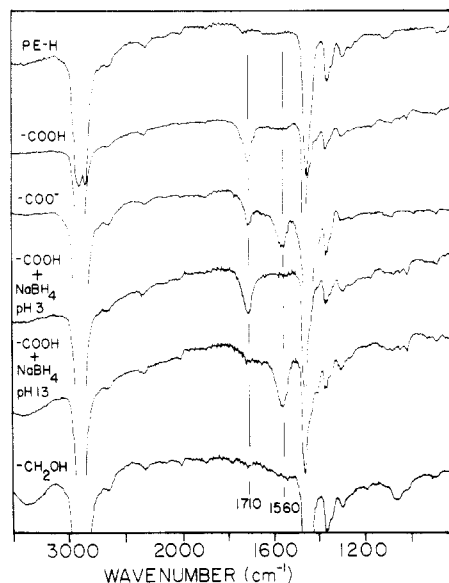
Figure 6. ATR-IR spectra of samples of polyethylene: following extraction (PE-H); after oxidation (PE-COOH); after treatment with 1 N NaOH (PE-COO - ); following treatment with NaBH 4 , shown after equilibration of the surface at pH 3 and 13; following treatment with 1 M BH 3 ·THF (PE-CH 2 OH).
