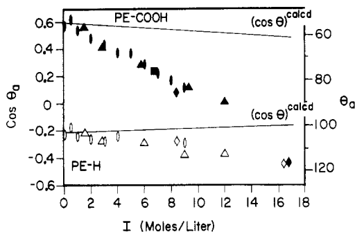
Figure 24. Effect of ionic strength ( I ) on \cos \theta_a for PE-H and PE-CO 2 H. Salts: (●, ○) NaClO 4 ; (▲, △) (NH 4 ) 2 SO 4 ; (■) NaI; (◆, ◇) AlCl 3 . The changes in \cos \theta_a predicted from changes in \gamma_{LV} alone (eq 12), using values of \gamma_{LV} for (NH 4 ) 2 SO 4 as representative, are shown for comparison.
