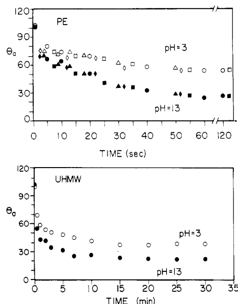
Figure 4. Advancing contact angle for water at pH 3 (HCl, open symbols) and pH 13 (NaOH, filled symbols) for samples of low-density polyethylene film (PE) and ultrahigh molecular weight polyethylene sheet (UHMW) oxidized for times indicated, using the standard procedure (see Text): (○, ●) unannealed; (□, ■) annealed 100 °C for 96 h; (◇, ◆) annealed 110.6 °C, 24 h; (▲, △) unannealed Monsanto K-2400-212 polyethylene. Extended oxidation of either material increases the roughness of the surface but does not change the contact angle at pH 3 or 13.
