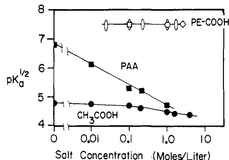
Figure 23. Dependence of the \text{pK}_a^{1/2} of PE- \text{CO}_2\text{H} on aqueous salt concentration: ( \diamond ) \text{NaNO}_3 ; ( \circ ) LiCl; ( \square ) \text{CaCl}_2 ; ( \circ ) NaCl. All solutions also contain 0.05 M buffer. Data for \text{CH}_3\text{CO}_2\text{H} 43 and polyacrylic acid (PAA) 44 in aqueous NaCl are also shown.
