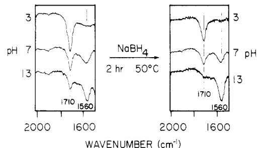
Figure 12. ATR-IR spectra of PE-COOH (left) and PE-CO 2 H after treatment with NaBH 4 to remove ketone and aldehyde functionality (right) at several values of pH.
