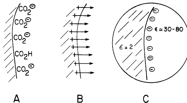
Figure 25. Schematic diagrams illustrating three possible factors influencing the ionization of surface-bound carboxylic acids. (A) ion-ion interactions; (B) dipolar interactions between the functional groups on the surface and the solvent; (C) the low "average" dielectric constant of the PE-CO 2 H/H 2 O interface.
