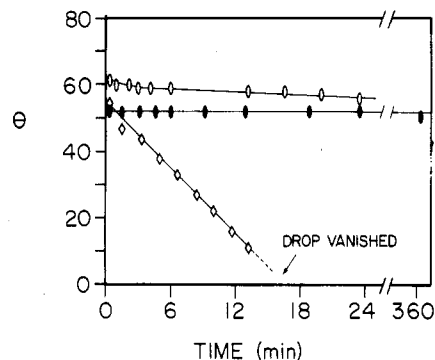
Figure 14. Variation in the measured value of \theta as a function of the interval between application of the drop to the surface and the measurement. Data points are for typical single drops; (●) applied and measured under air saturated with water vapor (100% relative humidity); (○) applied at ambient humidity and then raised to 100% relative humidity; (◇) applied and kept at ambient humidity.
