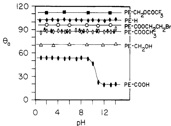
Figure 11. Dependence of \theta_a on pH (unbuffered solutions; pH adjusted with NaOH or HCl) for PE-COOH and several derivatives. The PE-CO 2 CH 3 samples were made as follows: (○) by acid-catalyzed esterification; (◐) by reaction with diazomethane; (◑) by reaction of PE-COCl and CH 3 OH.
