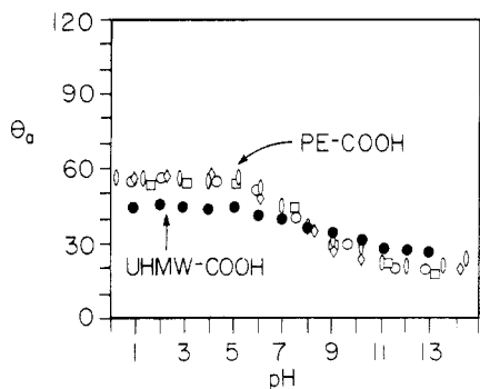
Figure 15. Dependence of \theta_a on pH for PE-CO 2 H with various pretreatments: (○) dry film; (□) film equilibrated at pH 13 (NaOH) for 3 h, then washed in distilled water for 5 min, and dried in air for 30 min; (◇) film equilibrated at pH 1 (HCl) for 3 h then washed, and dried as above; (○) film subjected to five cycles between pH 1 and 13 (5 min each), then washed in distilled water for 5 min, and dried. The results for UHMW-CO 2 H (no pretreatment) are included (●).
