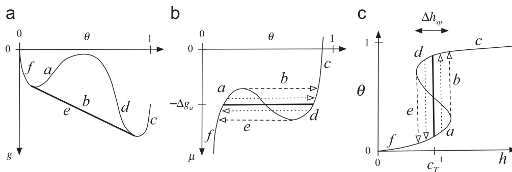
Fig. 3. Effects of lateral forces on adsorption. (a) Gibbs free energy per site g versus dimensionless filling \Theta of adsorbate. The homogeneous free energy g_{\text{hom}} (thin solid line) is made convex by a common tangent construction (thick solid line), which corresponds to phase separation into high and low density regions (neglecting interphasial tension). (b) Chemical potential \mu per site for homogeneous (thin solid) and phase separated (thick solid) states. (c) The corresponding filling fraction versus relative humidity h for quasi-equilibrium between the adsorbate and vapor. Hysteresis during adsorption ( a \rightarrow b \rightarrow c in Fig. 10) or desorption ( d \rightarrow e \rightarrow f ) results from the delay in phase separation due to either nucleation (dotted lines) or spinodal decomposition (dashed lines).
