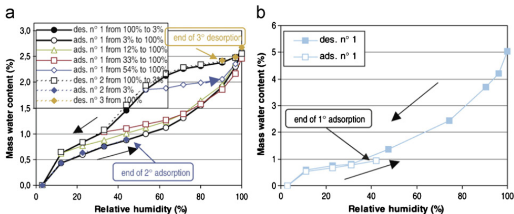
Fig. 1. Experimental data for isothermal water–vapor desorption and sorption cycles in concrete at different temperatures. (a) Pronounced hysteresis at T=23 °C. (b) Suppressed hysteresis at T=44 °C. [Reproduced from Fig. 2(e) and (g) of Baroghel-Bouny (2007) with permission.]
