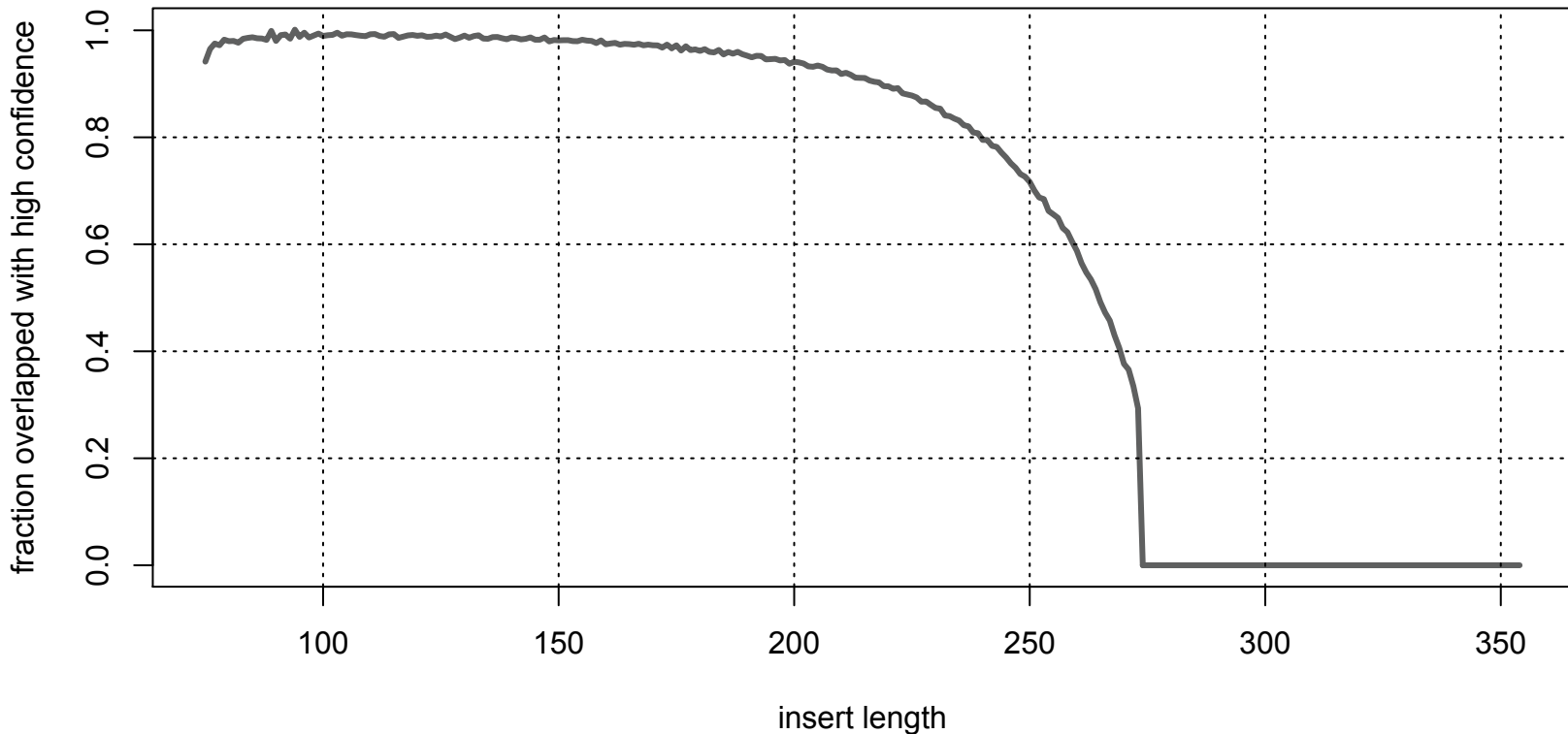
Overlapping success by insert length, for 2x143 bp, Sept09 data
