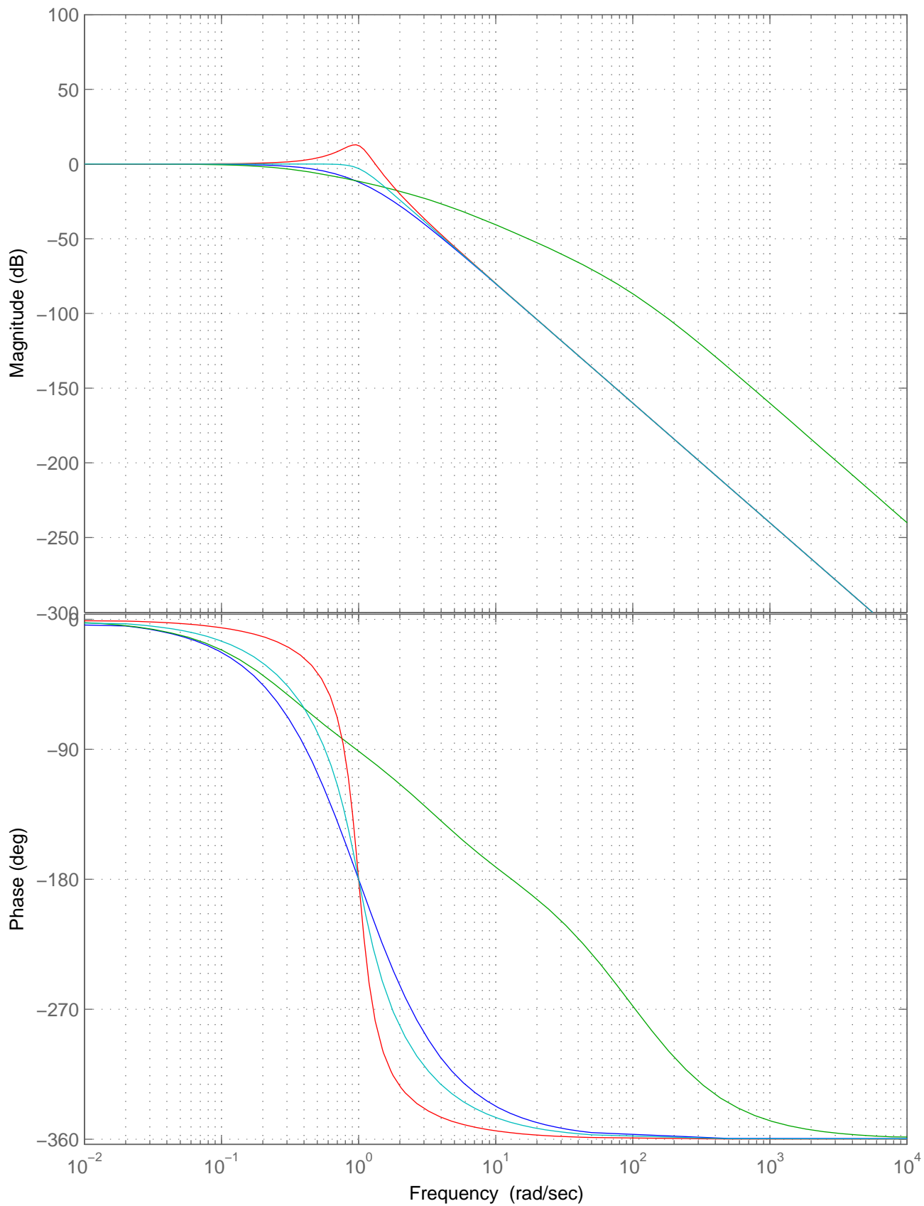
Bode Diagram
