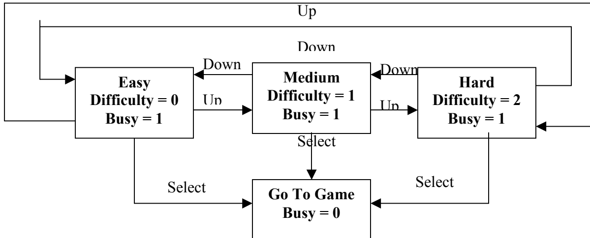
Figure 5. Menu Minor FSM
