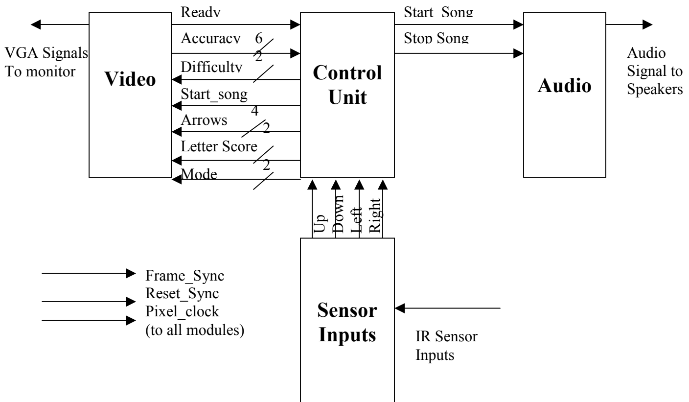
Figure 2. High Level Block Diagram
