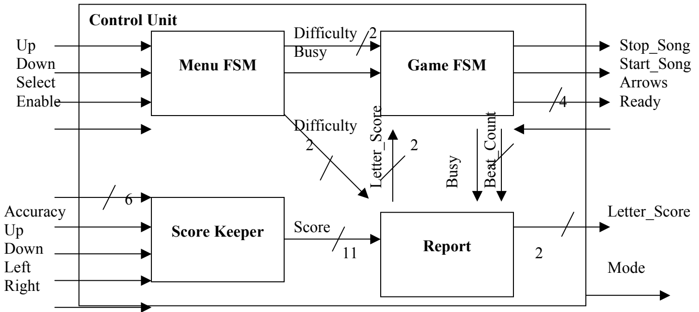
Figure 3. Control Unit Block Diagram
