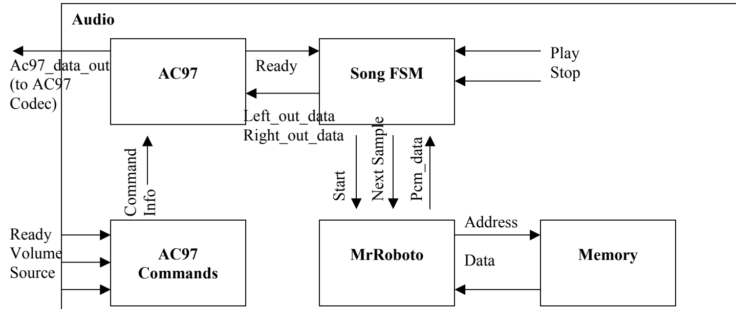
Figure 9. Audio Component Block Diagram
