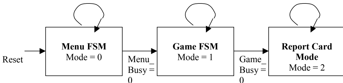
Figure 4. Control Unit Major FSM Diagram
