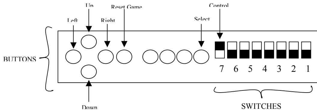
Figure 1. Labkit Interface
