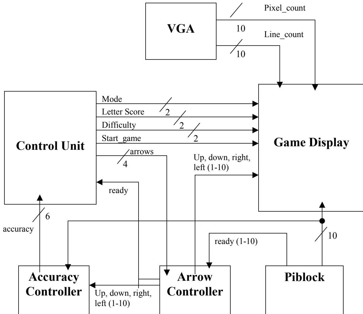
Figure 7. The Video Component Block Diagram
