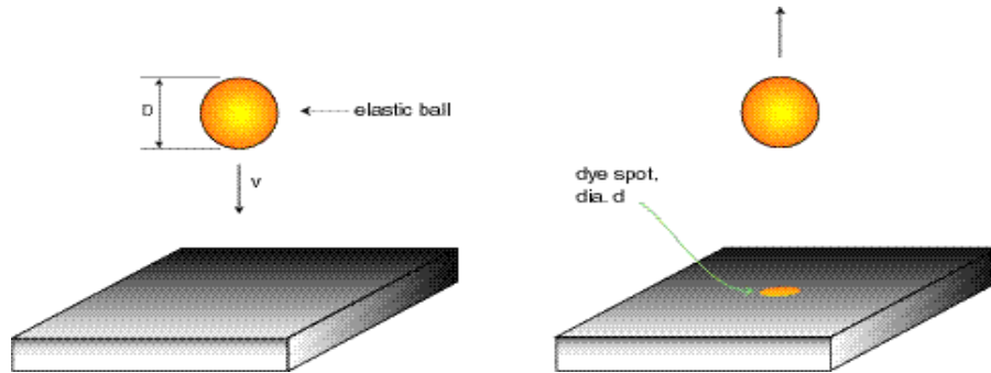
Fig. 3.1: A freshly dyed elastic ball leaving imprint after impact with rigid wall.
