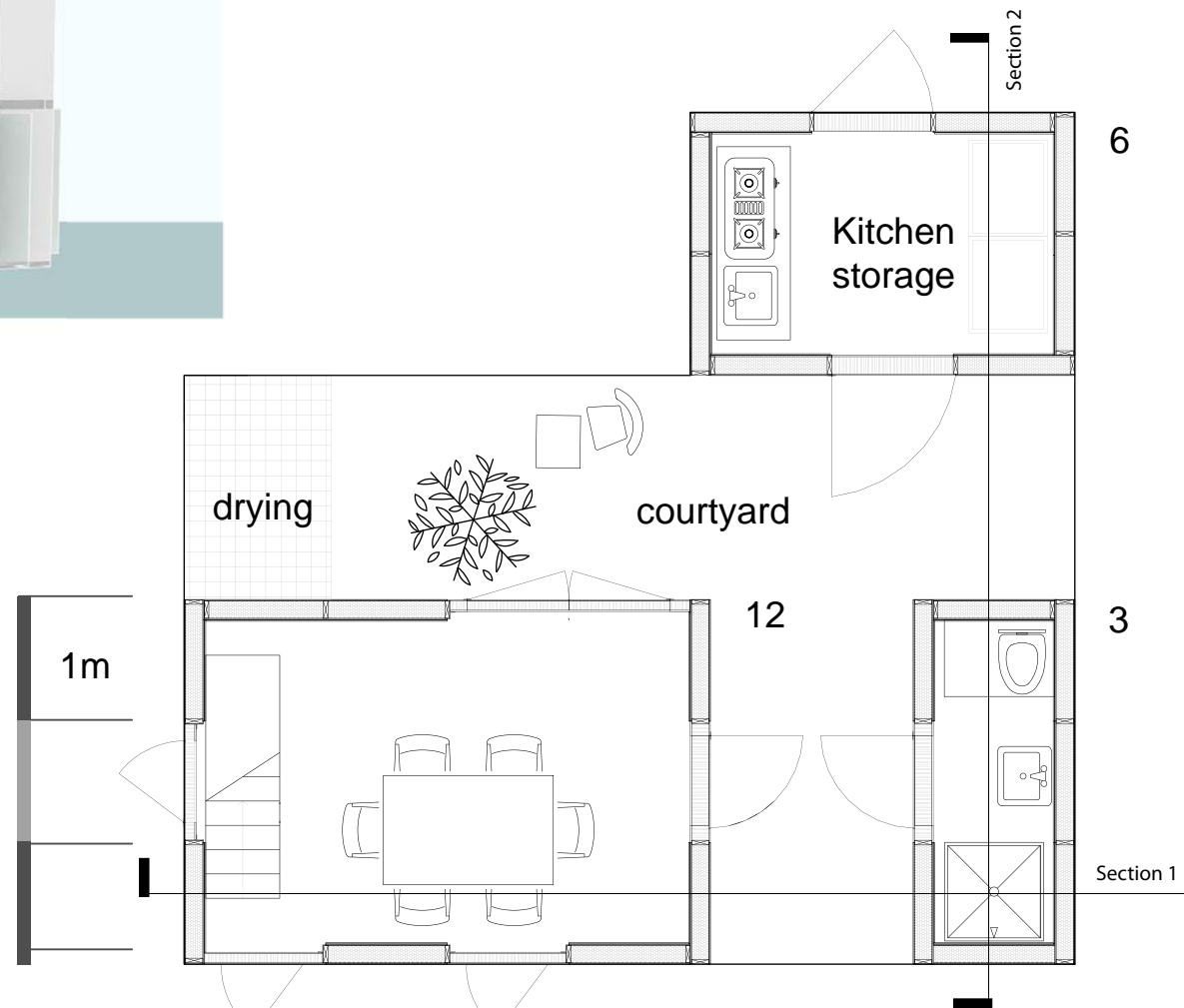
Ground floor plan 1:60
