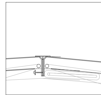
C OPERABLE ROOF PANEL (CLOSED)
