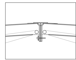
B STANDARD RIDGE CONNECTION
