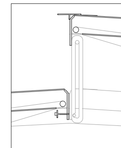
D OPERABLE ROOF PANEL OPEN
