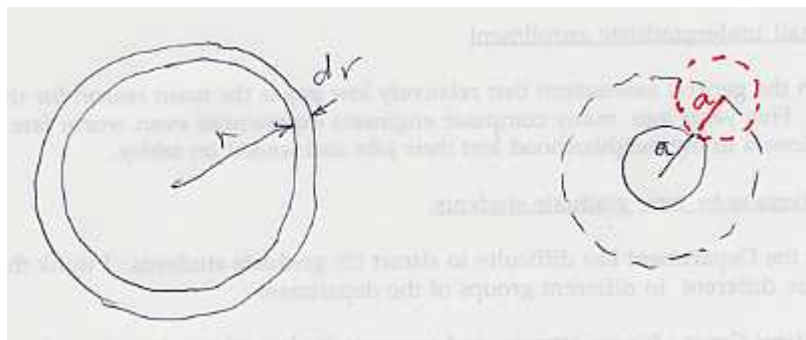
Figure 2.7.1: Left: A spherical shell. Right: Two spherical particles in collision.
